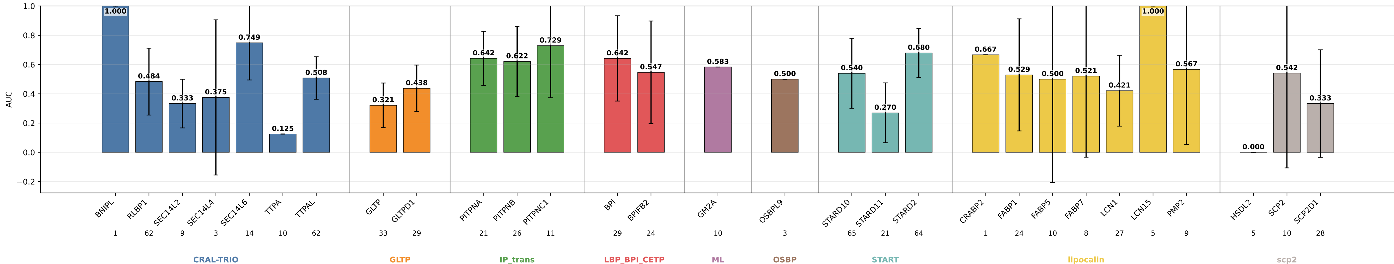
dh_s15_mbw_lipprop AUC by subgroup dh_s15_mbw_lipprop | class weights | lr=0.0001 | weight_decay=0.01 | final_m=4 | final_dropout=0.1 | hiddim=8 | heads=8 | batch=16 | ep=120 | seeds=0,1,2,3,4
