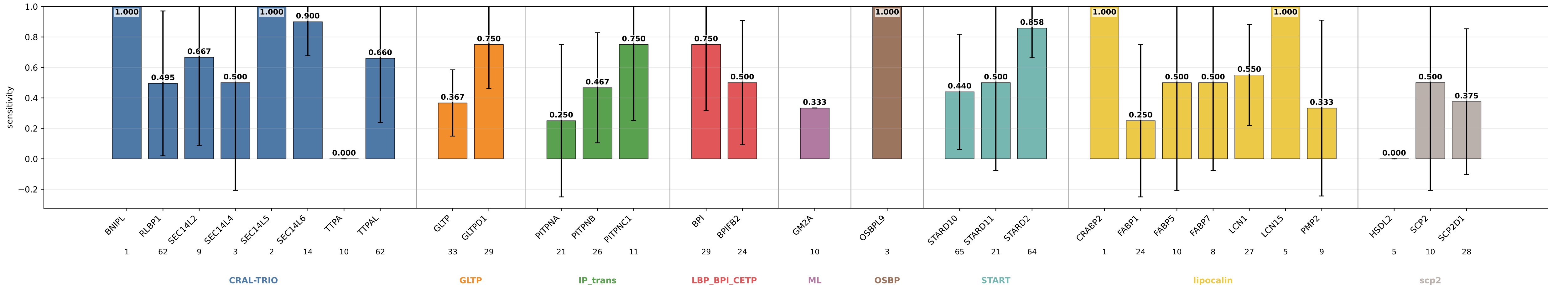
dh_s15_mbw_lipprop sensitivity by subgroup dh_s15_mbw_lipprop | class weights | lr=0.0001 | weight_decay=0.01 | final_m=4 | final_dropout=0.1 | hiddim=8 | heads=8 | batch=16 | ep=120 | seeds=0,1,2,3,4
