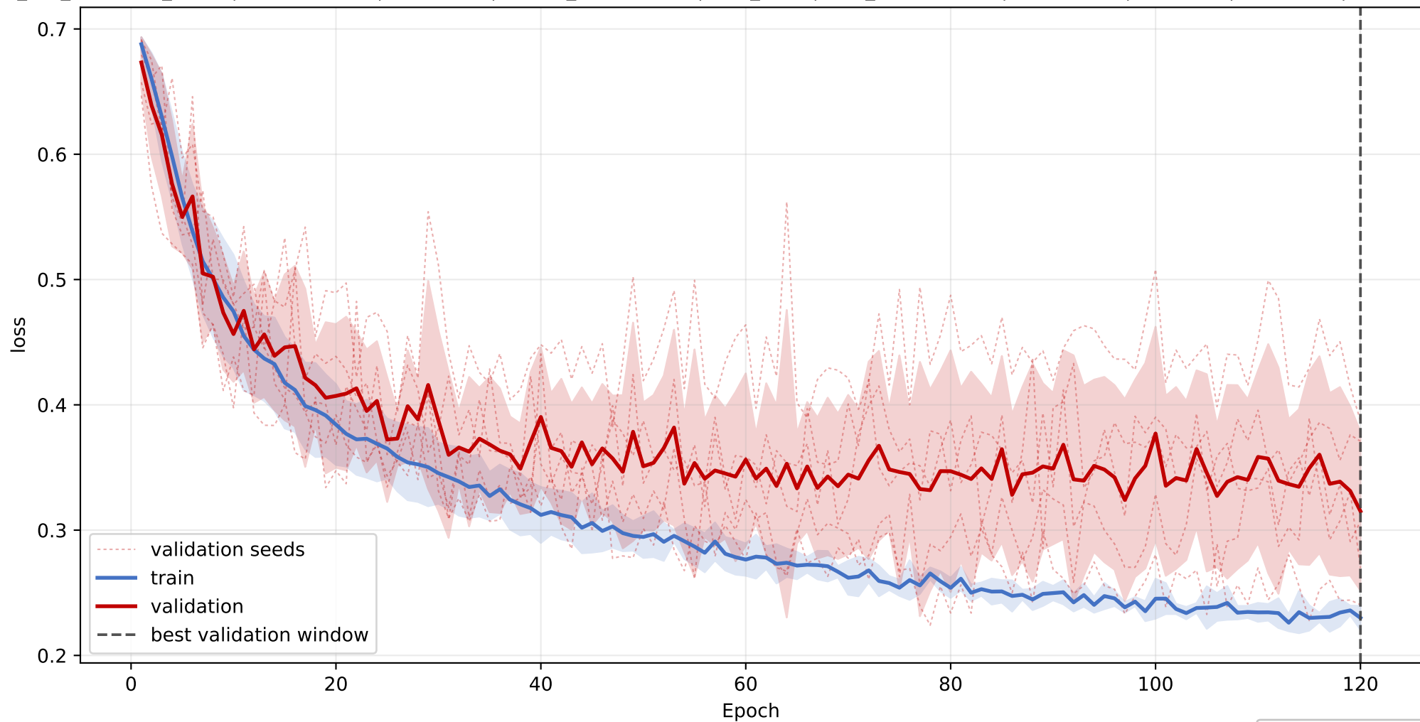
species15: mean loss learning curve across seeds
