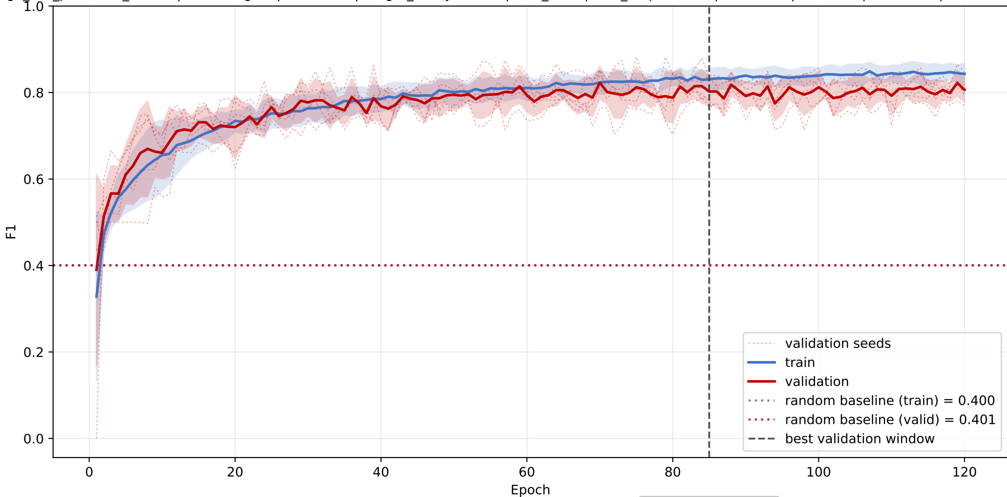
species15: mean F1 learning curve across seeds
