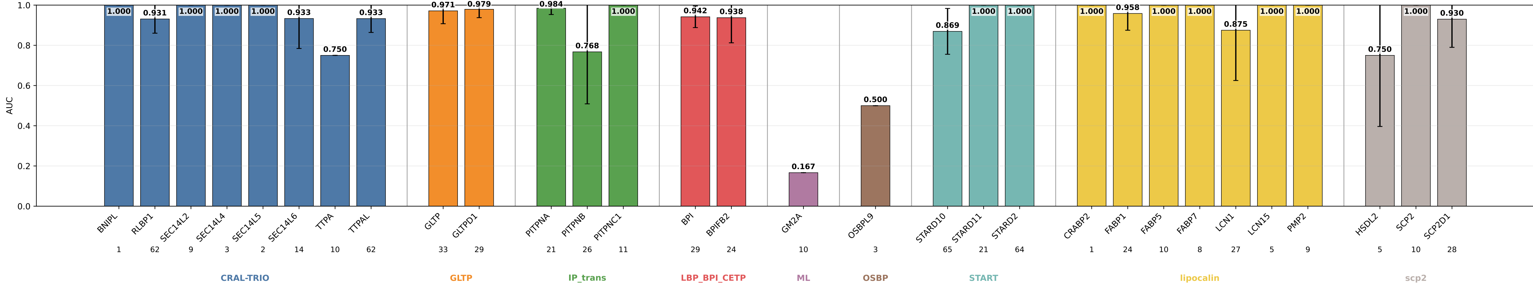
ge_s15_prothid32_wd1e5 AUC by subgroup ge_s15_prothid32_wd1e5 | class weights | lr=0.0001 | weight_decay=1e-05 | final_m=4 | final_dropout=0.1 | hiddim=8 | heads=8 | batch=16 | ep=120 | seeds=0,1,2,3,4
