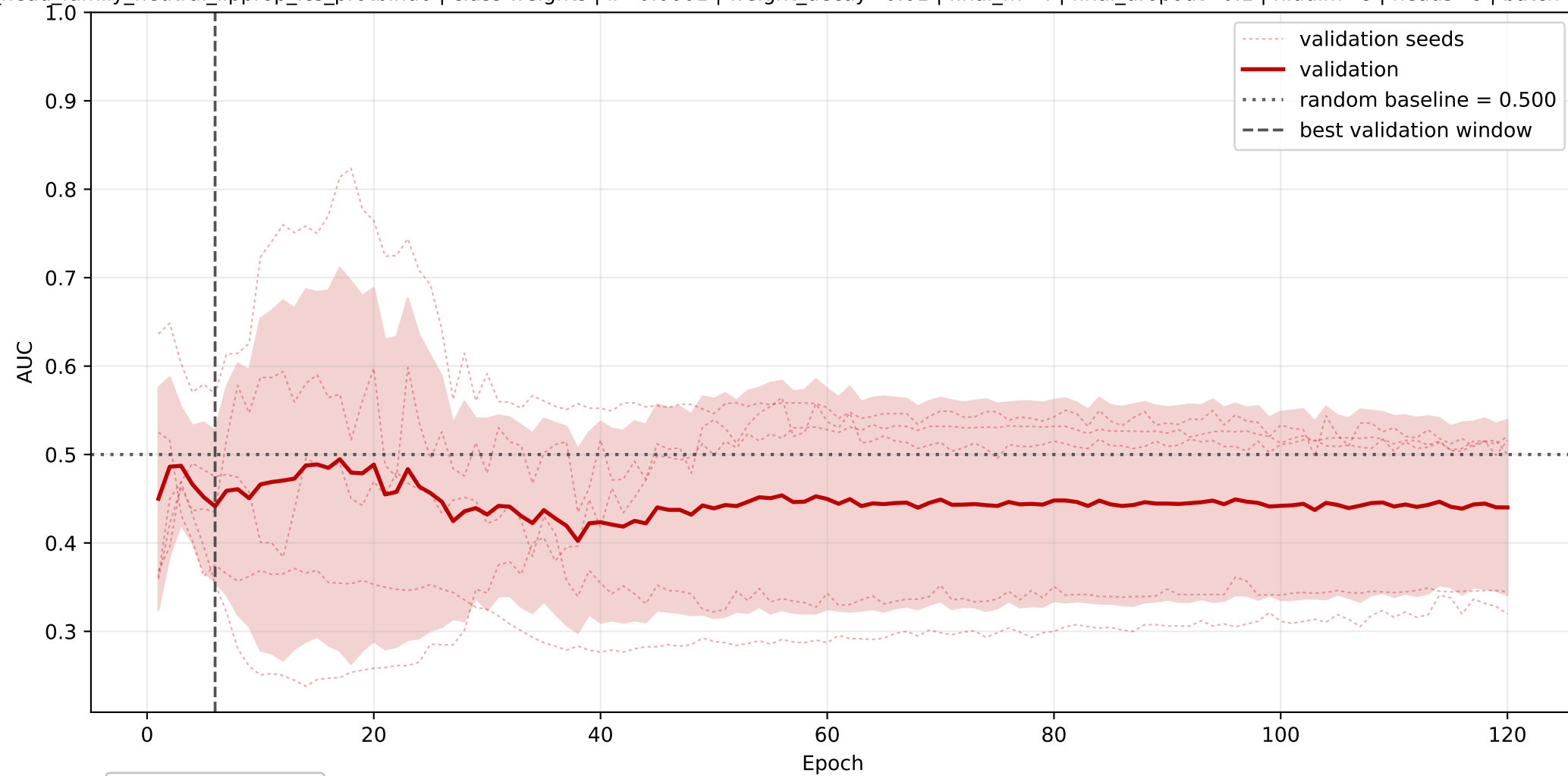
sphingolipids: mean AUC learning curve across seeds
