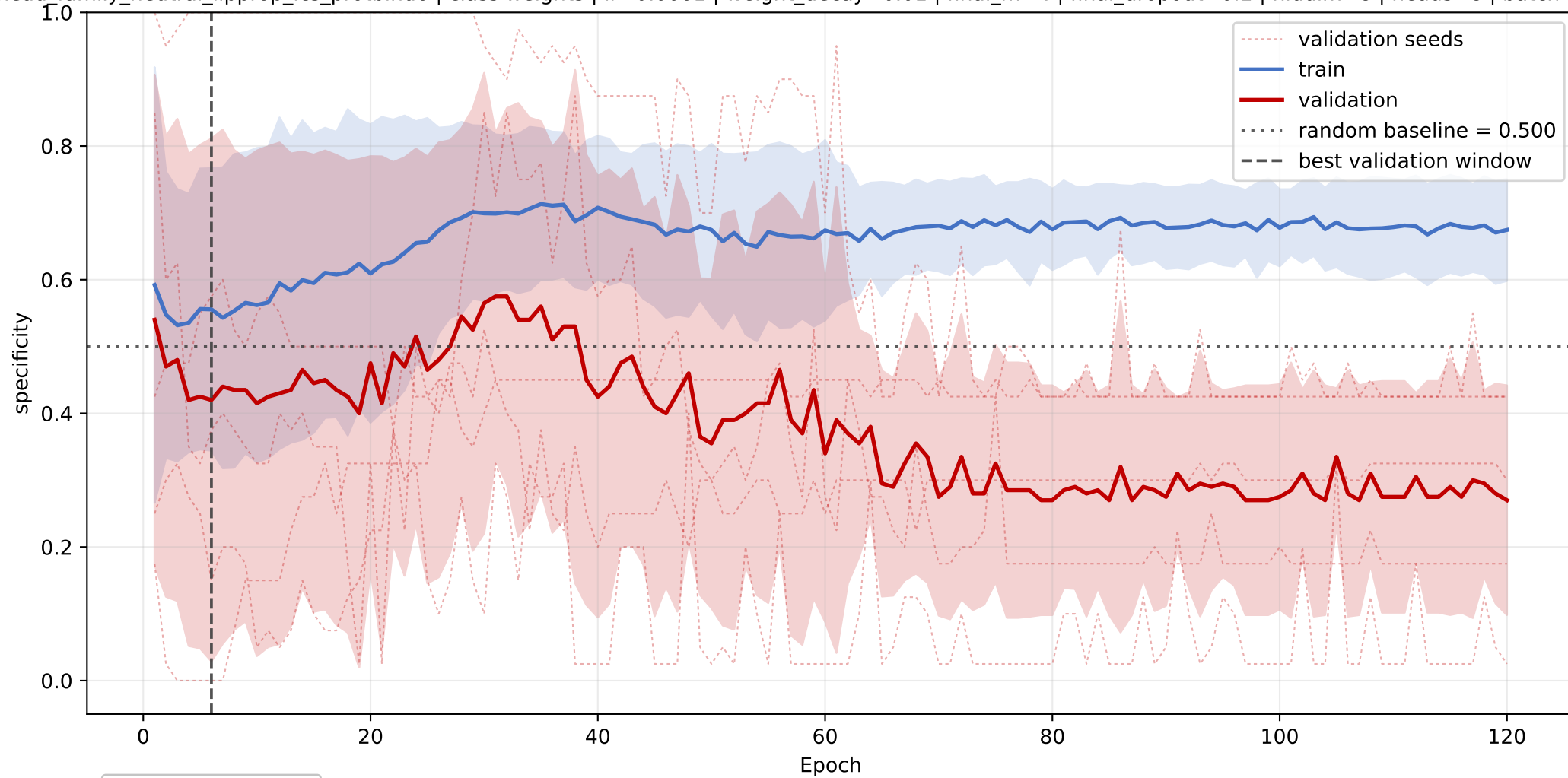
sphingolipids: mean specificity learning curve across seeds
