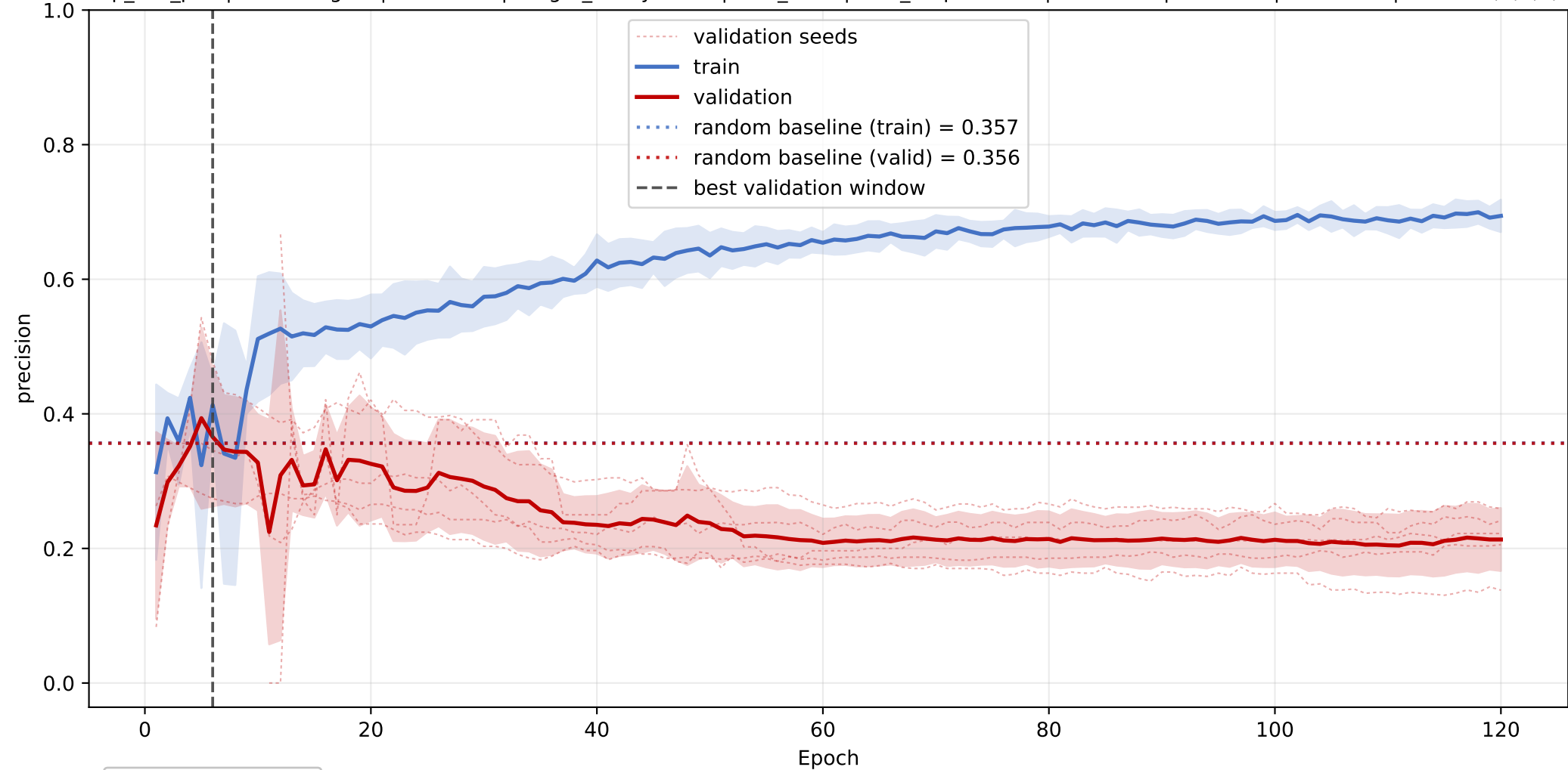
PC: mean precision learning curve across seeds
