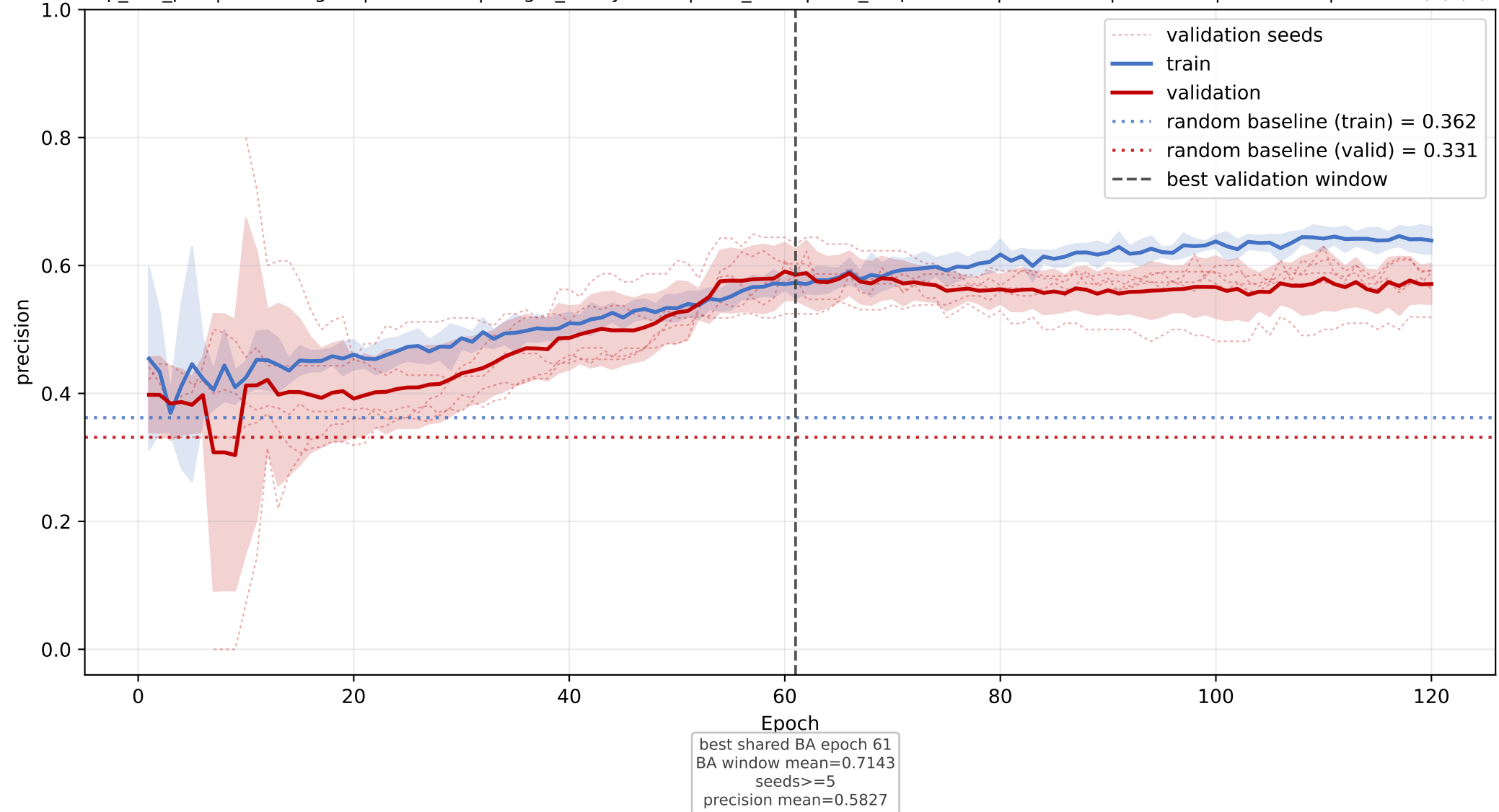
PG: mean precision learning curve across seeds
