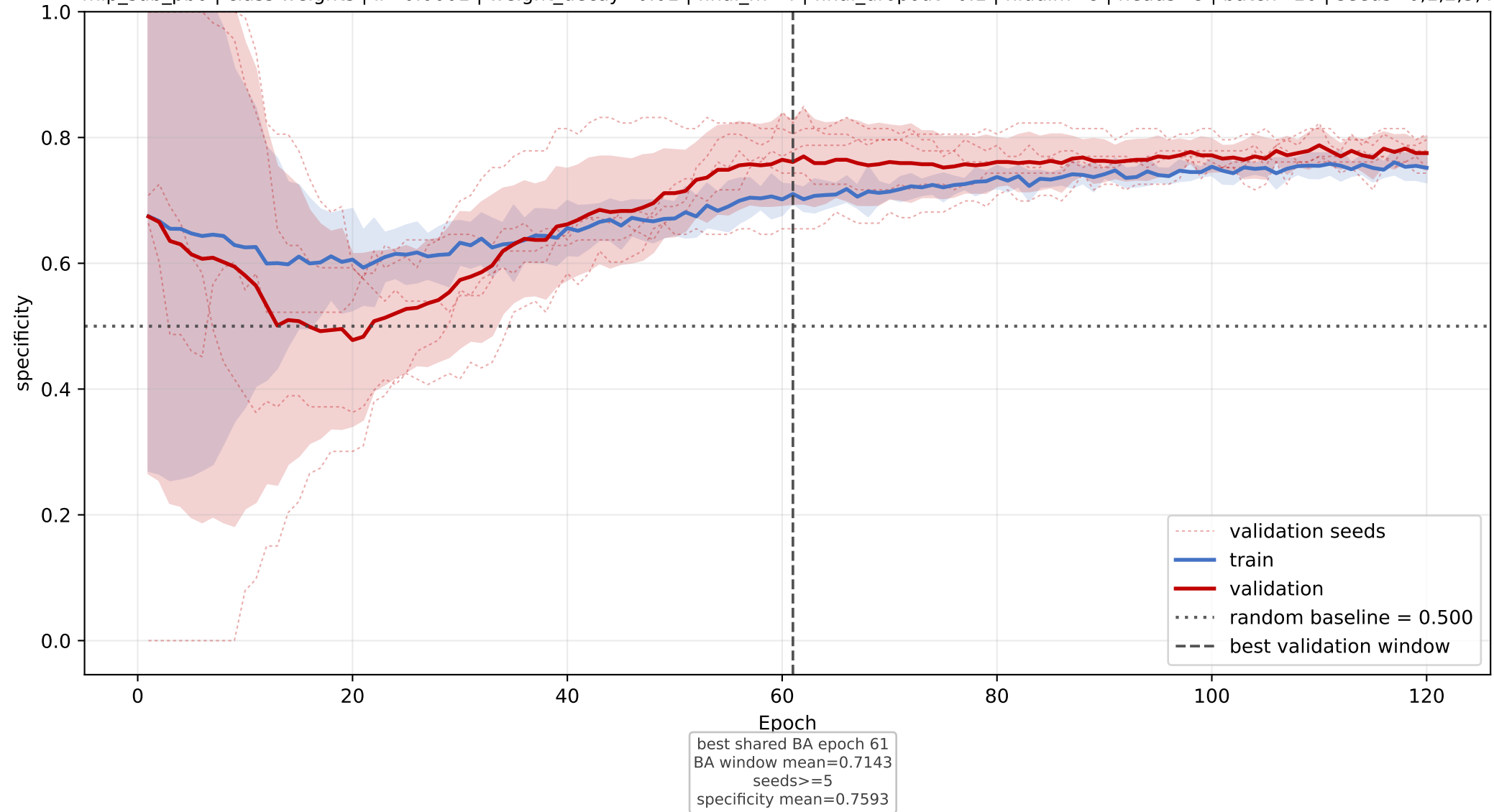
PG: mean specificity learning curve across seeds
