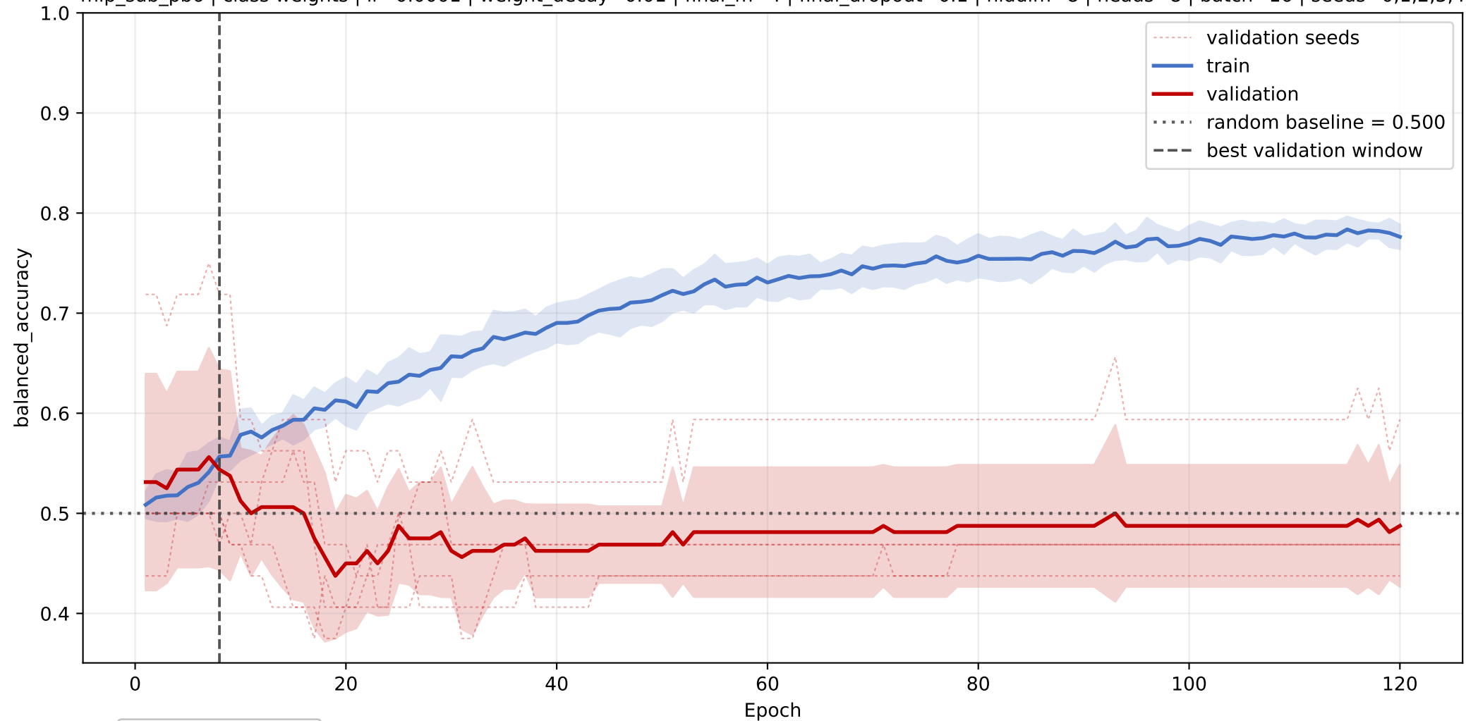
PI: mean balanced_accuracy learning curve across seeds
