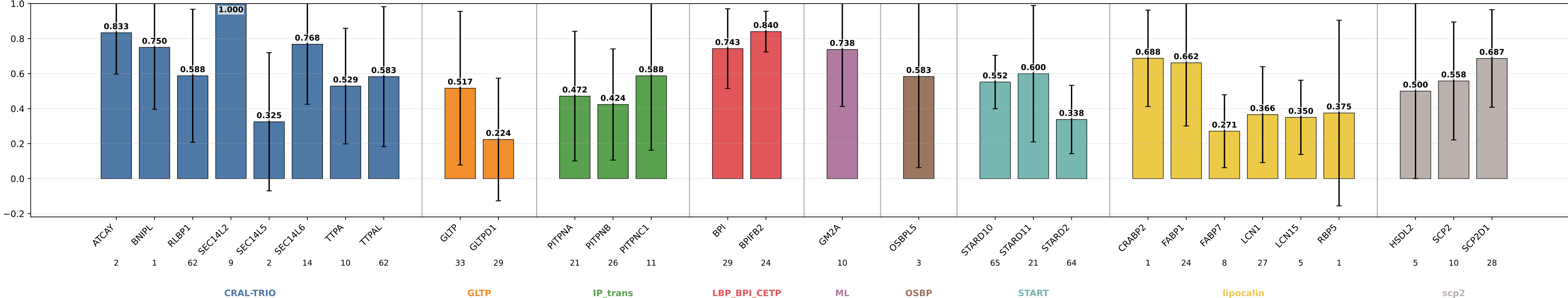
mlp_sub_pb6 AUC by subgroup mlp_sub_pb6 | class weights | lr=0.0001 | weight_decay=0.01 | final_m=4 | final_dropout=0.1 | hiddim=8 | heads=8 | batch=16 | ep=120 | seeds=0,1,2,3,4
