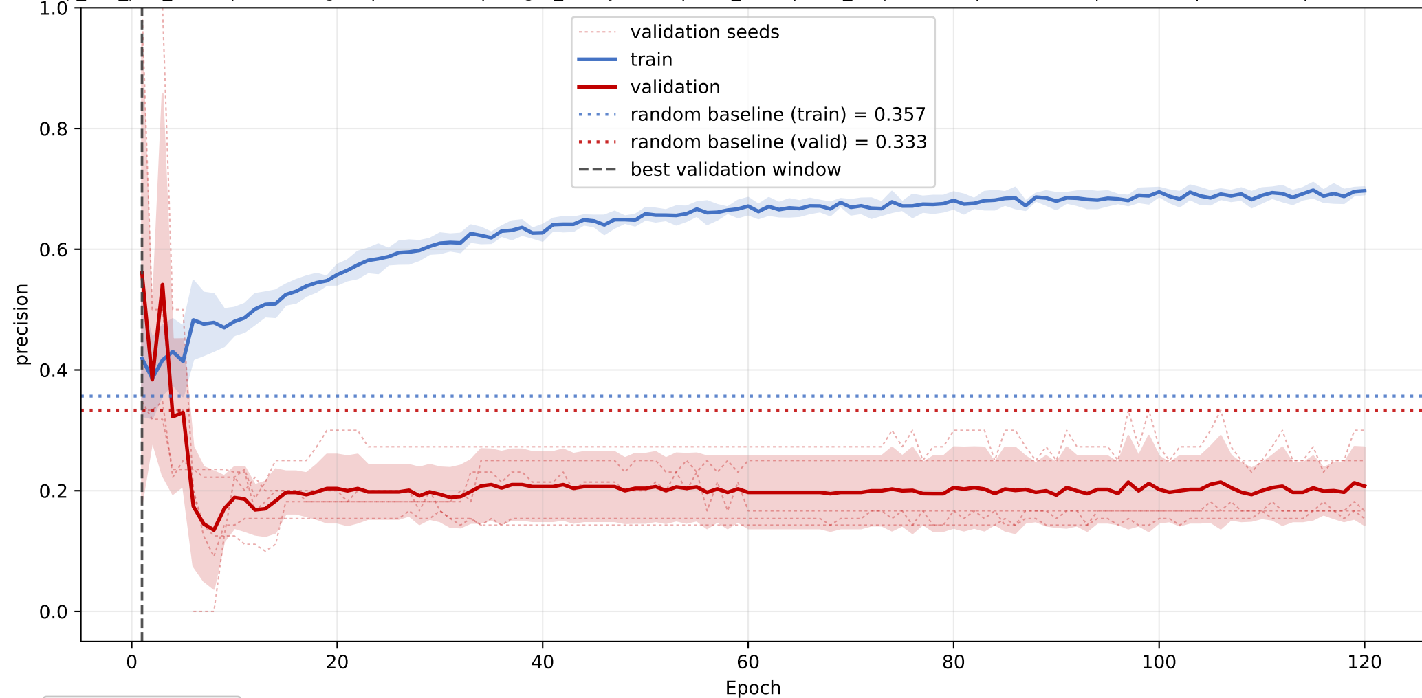
PS+PGP+DAG+TAG: mean precision learning curve across seeds
