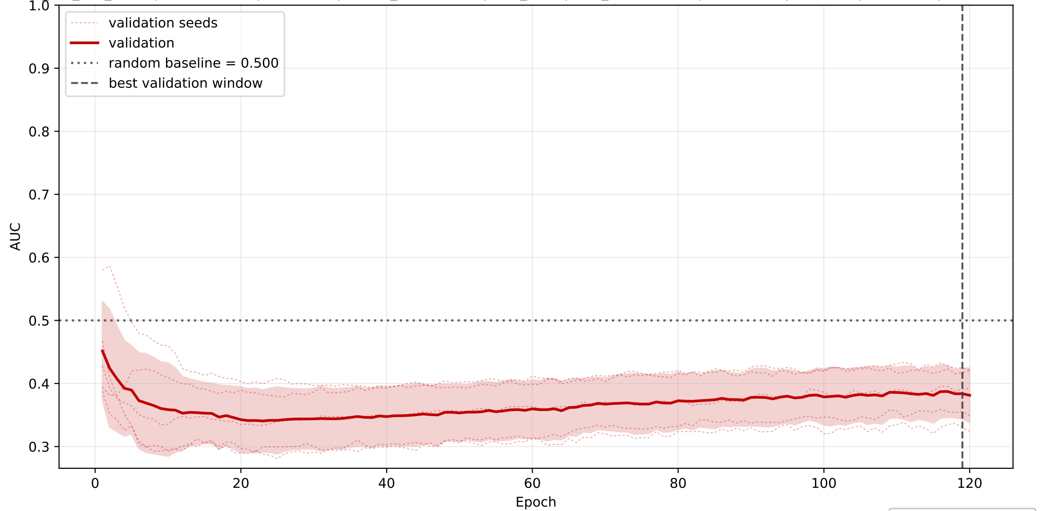
PC: mean AUC learning curve across seeds
