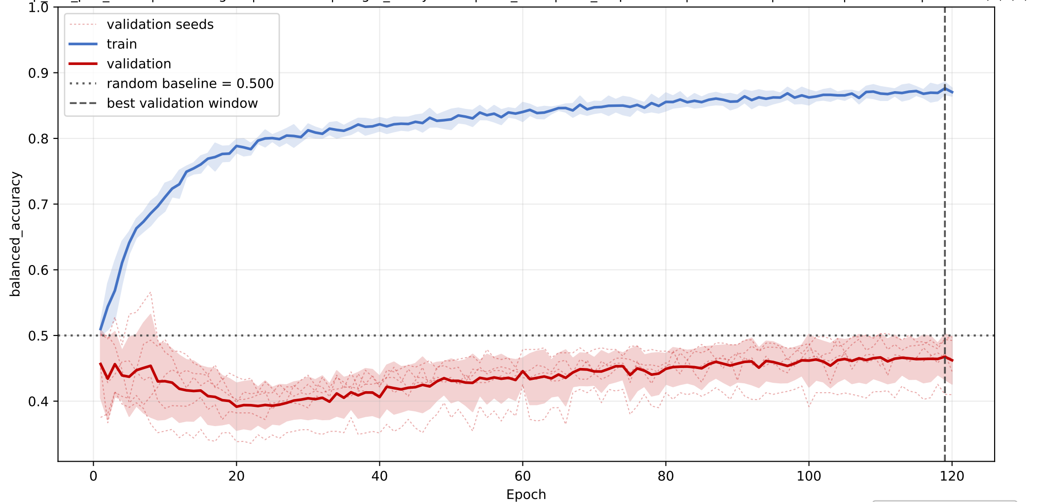
PC: mean balanced_accuracy learning curve across seeds
