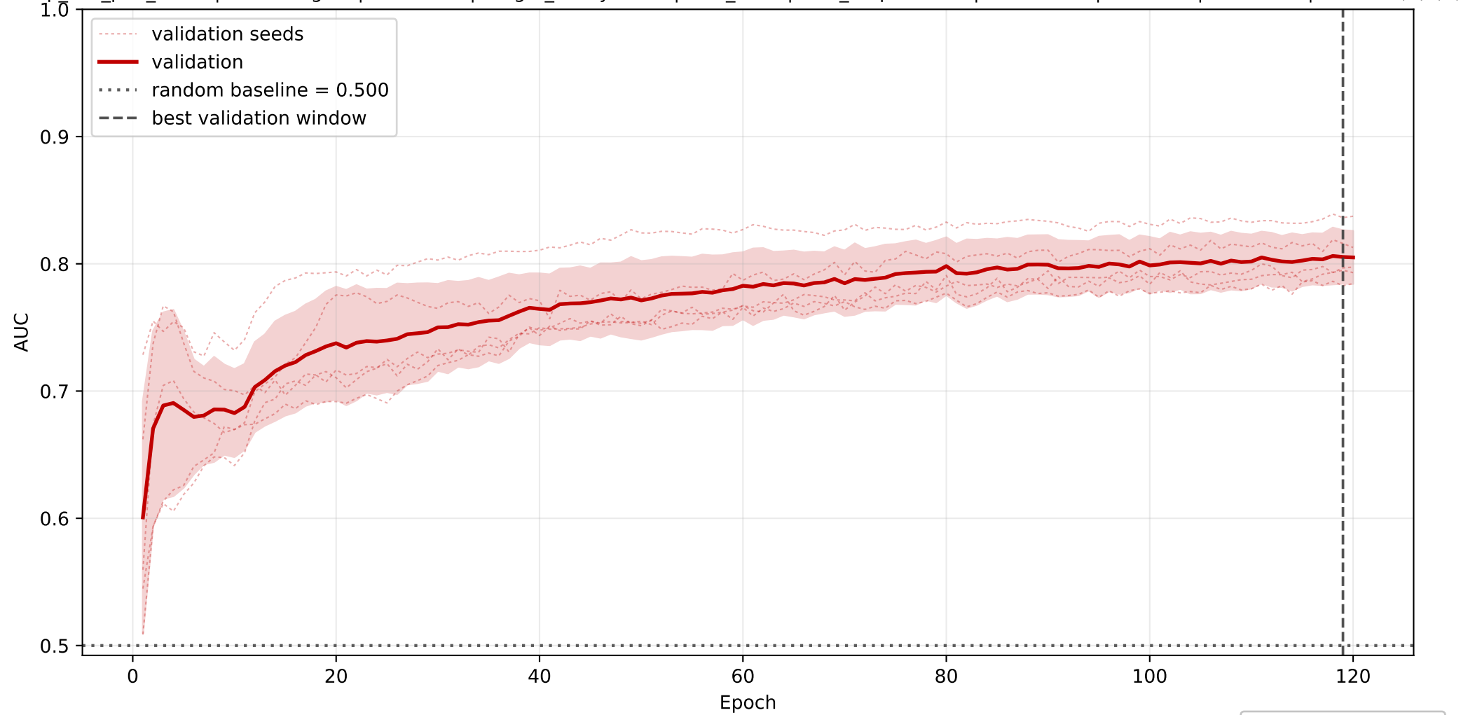
PG: mean AUC learning curve across seeds
