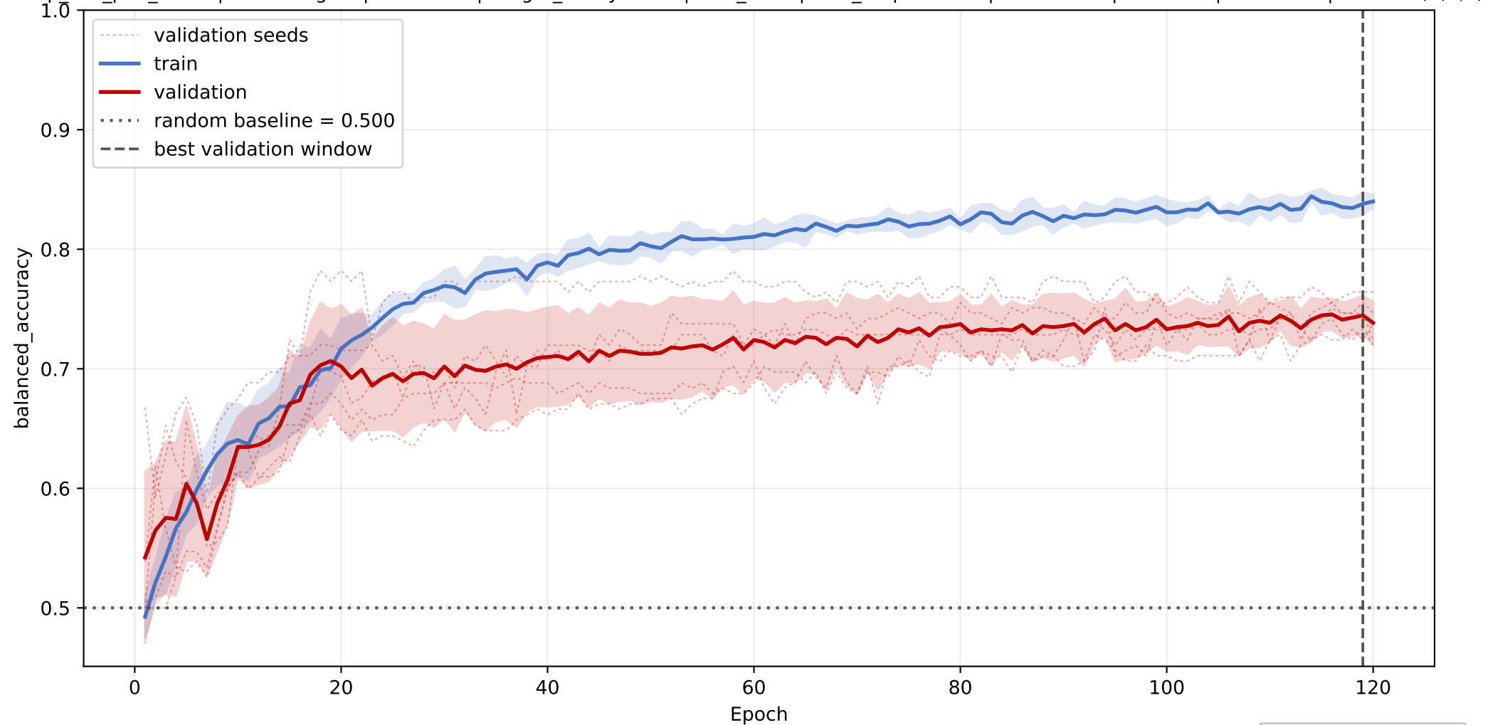
PG: mean balanced_accuracy learning curve across seeds
