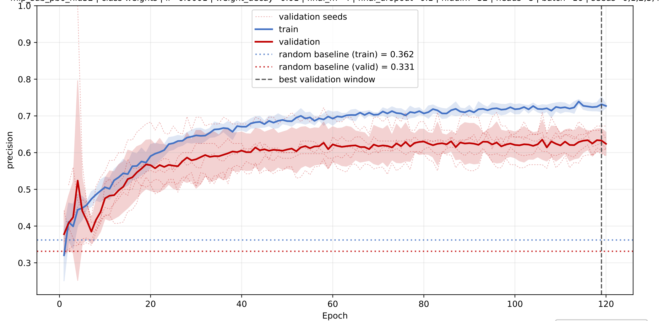
PG: mean precision learning curve across seeds
