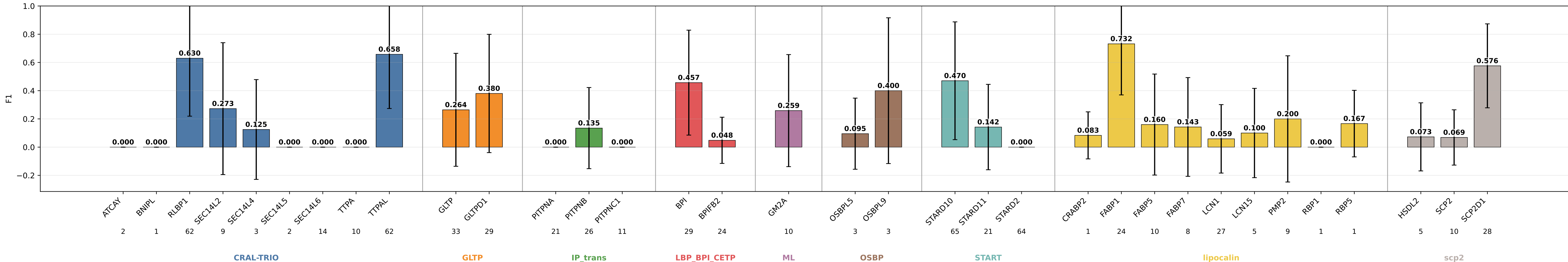
mlp_sub_pb6_hid32 F1 by subgroup mlp_sub_pb6_hid32 | class weights | lr=0.0001 | weight_decay=0.01 | final_m=4 | final_dropout=0.1 | hiddim=32 | heads=8 | batch=16 | ep=120 | seeds=0,1,2,3,4
