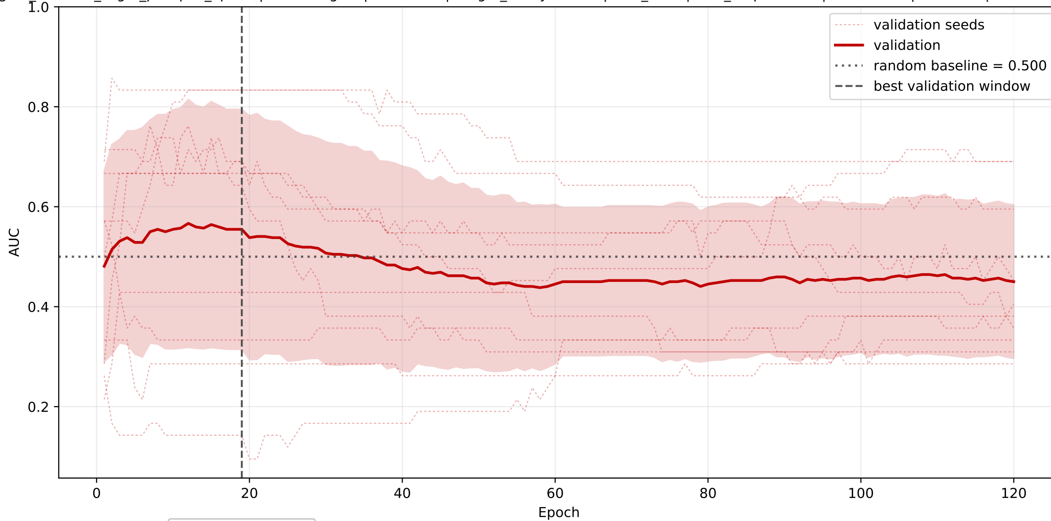
CerP+Hex2Cer+SHexCer_groups_glt: mean AUC learning curve across seeds
