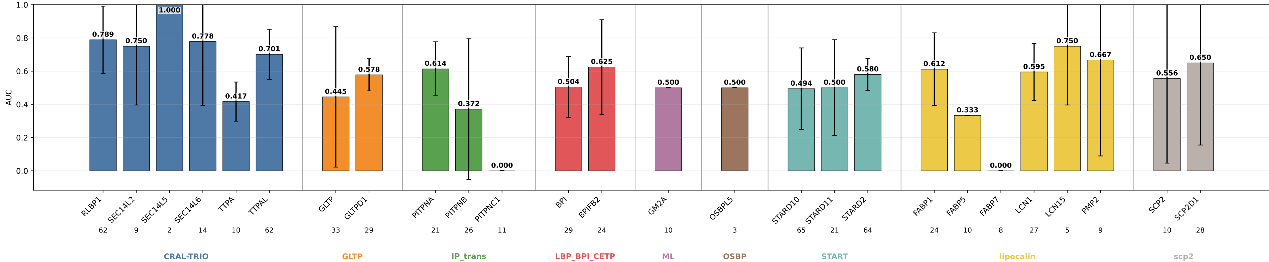
descriptors_head_family_neutral_lipprop_rand AUC by subgroup descriptors_head_family_neutral_lipprop_rand | class weights | lr=0.0001 | weight_decay=0.01 | final_m=4 | final_dropout=0.1 | hiddim=8 | heads=8 | batch=16 | ep=120 | seeds=0,1,2,3,4
