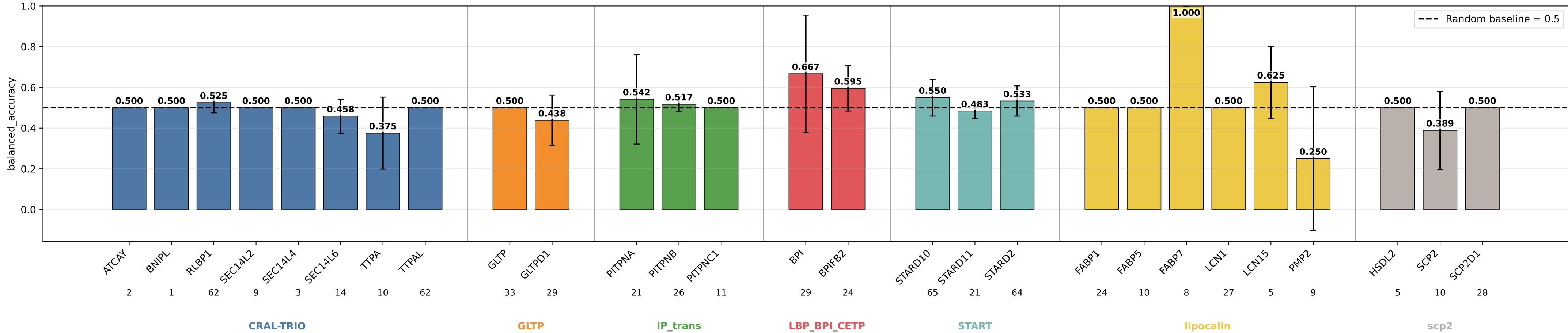
descriptors_head_family_neutral_lipprop_rand_protbind6 balanced_accuracy by subgroup descriptors_head_family_neutral_lipprop_rand_protbind6 | class weights | lr=0.0001 | weight_decay=0.01 | final_m=4 | final_dropout=0.1 | hiddim=8 | heads=8 | batch=16 | ep=120 | seeds=0,1,2,3,4
