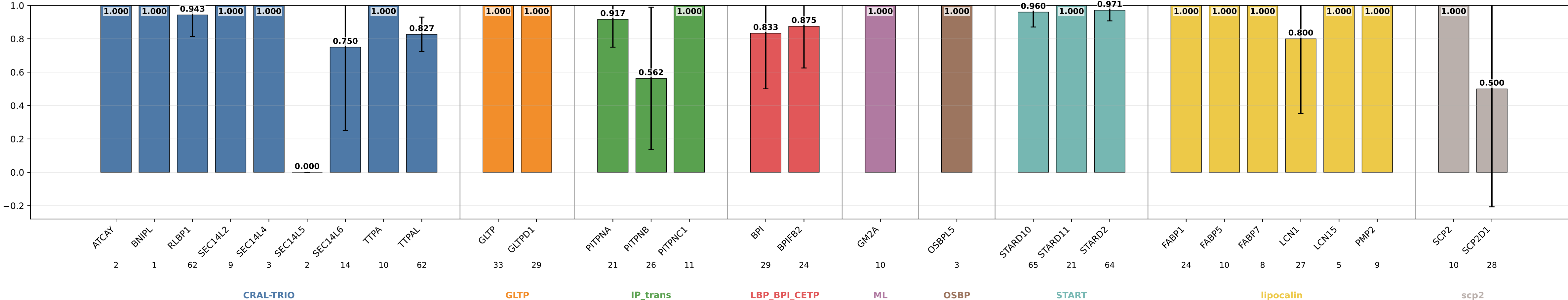
geometric_edge_mlp_protgeom_family_neutral_normalized_bilinear_fusion_bilinear_norm_esm3_protunion14_hid32_rand sensitivity by subgroup geometric_edge_mlp_protgeom_family_neutral_normalized_bilinear_fusion_bilinear_norm_esm3_protunion14_hid32_rand | class weights | lr=0.0001 | weight_decay=0.01 | final_m=4 | final_dropout=0.1 | hiddim=32 | heads=8 | batch=16 | ep=120 | seeds=0,1,2,3,4
