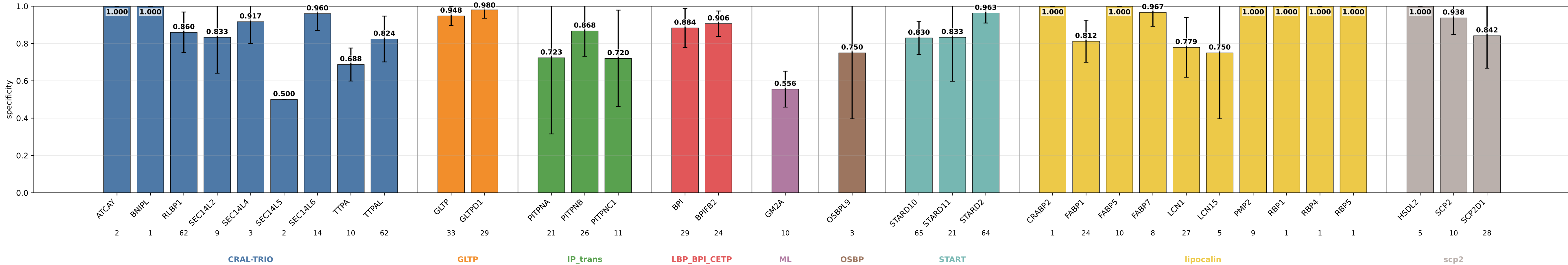
geometric_edge_mlp_protgeom_family_neutral_normalized_bilinear_fusion_bilinear_norm_esm3_protunion14_hid32_species15 specificity by subgroup geometric_edge_mlp_protgeom_family_neutral_normalized_bilinear_fusion_bilinear_norm_esm3_protunion14_hid32_species15 | class weights | lr=0.0001 | weight_decay=0.01 | final_m=4 | final_dropout=0.1 | hiddim=32 | heads=8 | batch=16 | ep=120 | seeds=0,1,2,3,4
