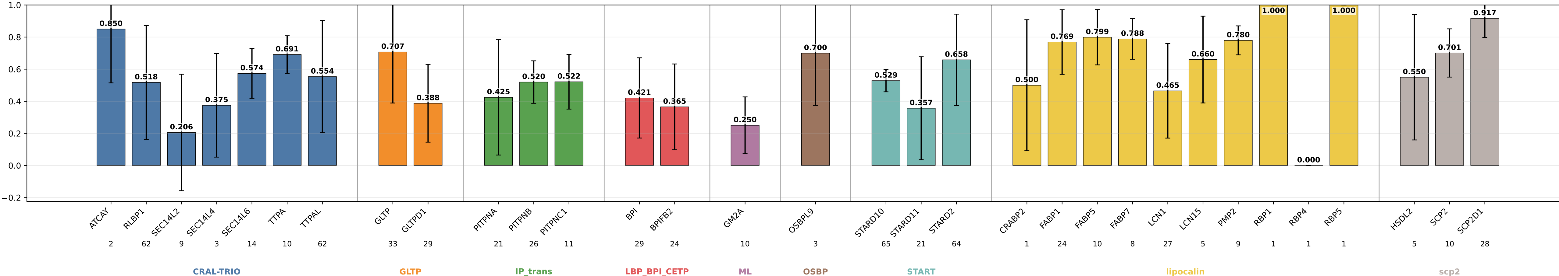
geometric_edge_mlp_protgeom_family_neutral_normalized_bilinear_fusion_bilinear_norm_lcs_esm3_protunion14_prothid32_pocketchem4 AUC by subgroup geometric_edge_mlp_protgeom_family_neutral_normalized_bilinear_fusion_bilinear_norm_lcs_esm3_protunion14_prothid32_pocketchem4 | class weights | lr=0.0001 | weight_decay=0.01 | final_m=4 | final_dropout=0.1 | hiddim=8 | heads=8 | batch=16 | ep=120 | seeds=0,1,2,3,4
