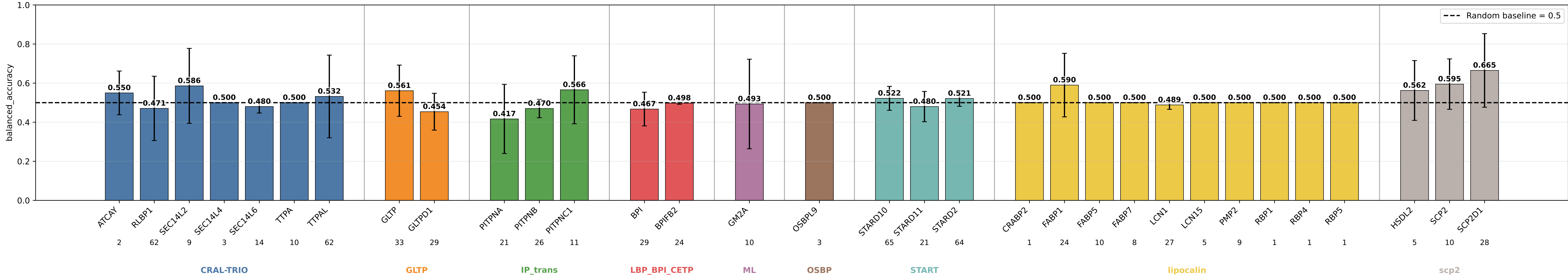
geometric_edge_mlp_protgeom_family_neutral_normalized_bilinear_fusion_bilinear_norm_lcs_esm3_protunion14_prothid32_rotneg balanced_accuracy by subgroup geometric_edge_mlp_protgeom_family_neutral_normalized_bilinear_fusion_bilinear_norm_lcs_esm3_protunion14_prothid32_rotneg | class weights | lr=0.0001 | weight_decay=0.01 | final_m=4 | final_dropout=0.1 | hiddim=8 | heads=8 | batch=16 | ep=120 | seeds=0,1,2,3,4
