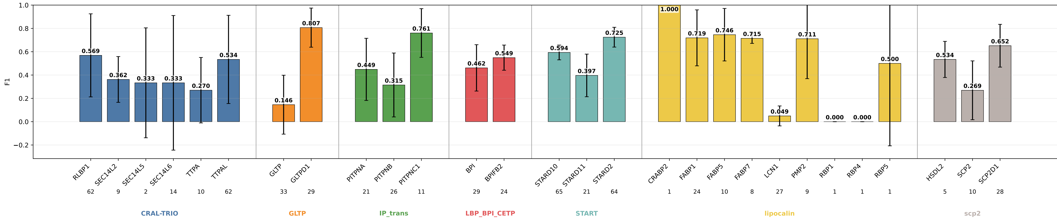
geometric_edge_mlp_protgeom8_normalized_dro F1 by subgroup geometric_edge_mlp_protgeom8_normalized_dro | class weights | lr=0.0001 | weight_decay=0.01 | final_m=4 | final_dropout=0.1 | hiddim=8 | heads=8 | batch=16 | ep=120 | seeds=0,1,2
