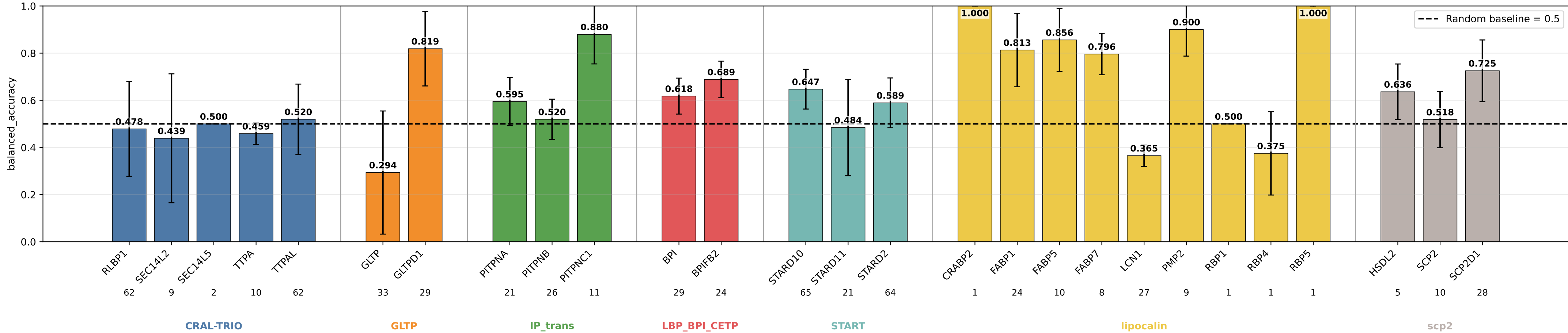
geometric_edge_mlp_protgeom8_normalized_dro balanced_accuracy by subgroup geometric_edge_mlp_protgeom8_normalized_dro | class weights | lr=0.0001 | weight_decay=0.01 | final_m=4 | final_dropout=0.1 | hiddim=8 | heads=8 | batch=16 | ep=120 | seeds=0,1,2
