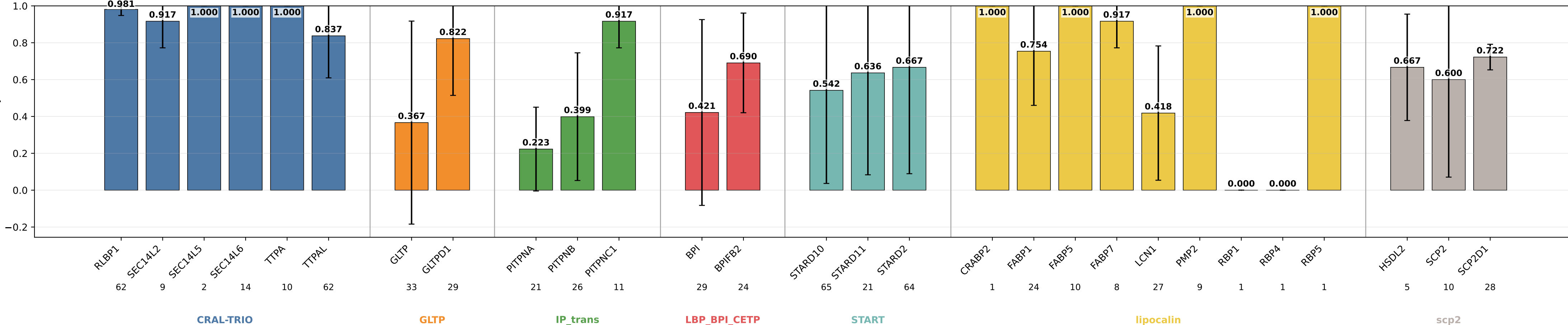
geometric_edge_mlp_protgeom_family_neutral_dro sensitivity by subgroup geometric_edge_mlp_protgeom_family_neutral_dro | class weights | lr=0.0001 | weight_decay=0.01 | final_m=4 | final_dropout=0.1 | hiddim=8 | heads=8 | batch=16 | ep=120 | seeds=0,1,2
