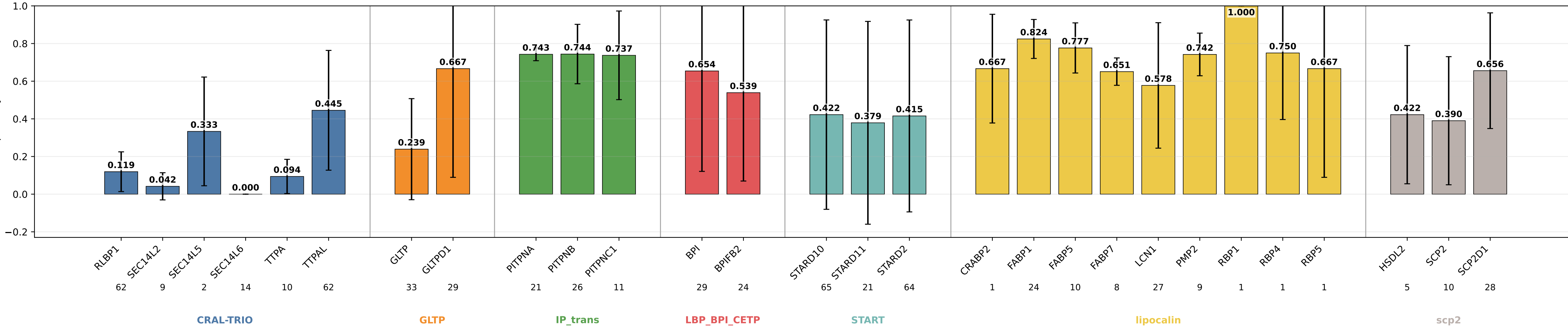
geometric_edge_mlp_protgeom_family_neutral_dro specificity by subgroup geometric_edge_mlp_protgeom_family_neutral_dro | class weights | lr=0.0001 | weight_decay=0.01 | final_m=4 | final_dropout=0.1 | hiddim=8 | heads=8 | batch=16 | ep=120 | seeds=0,1,2
