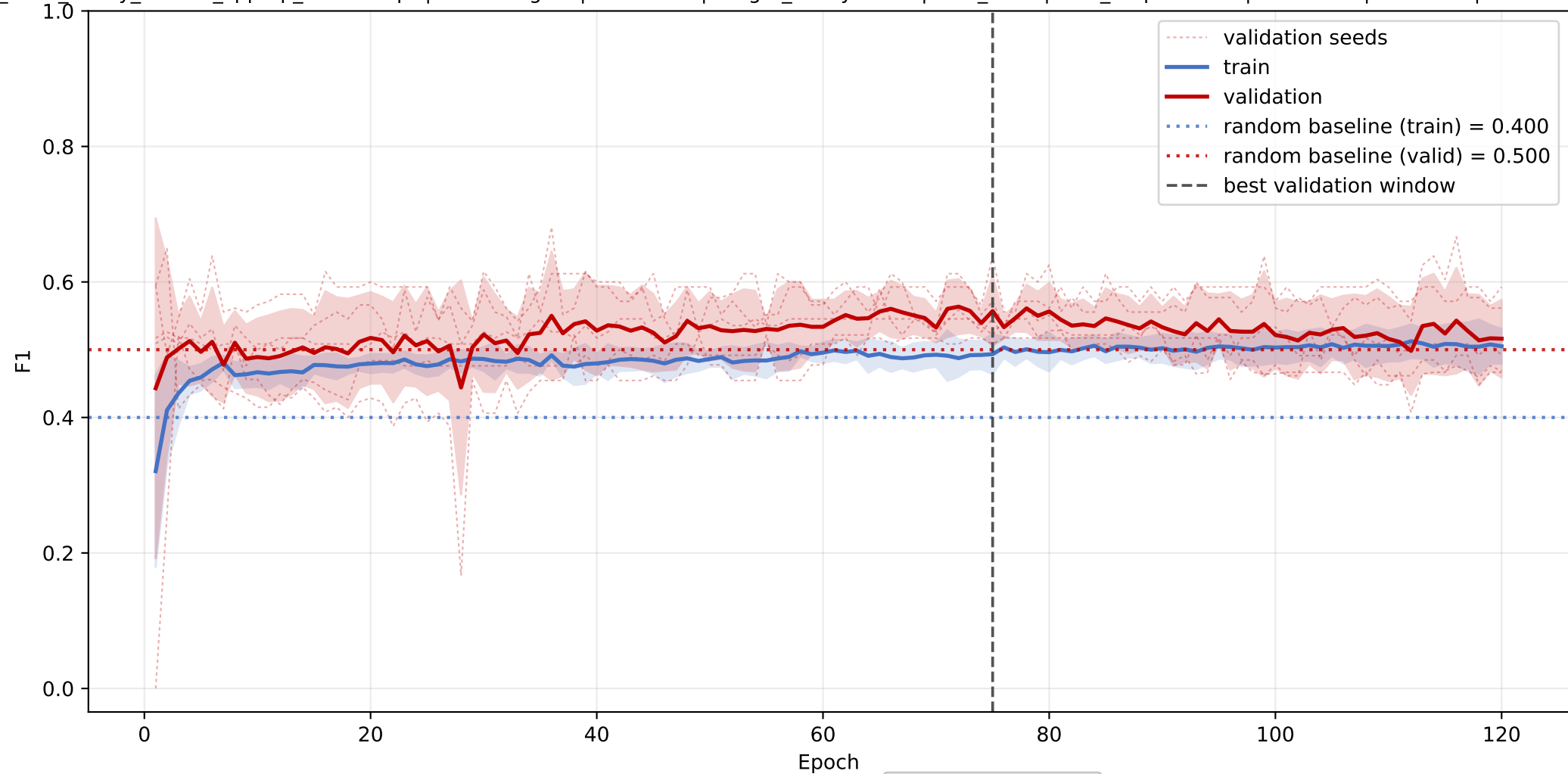
GLTP: mean F1 learning curve across seeds
