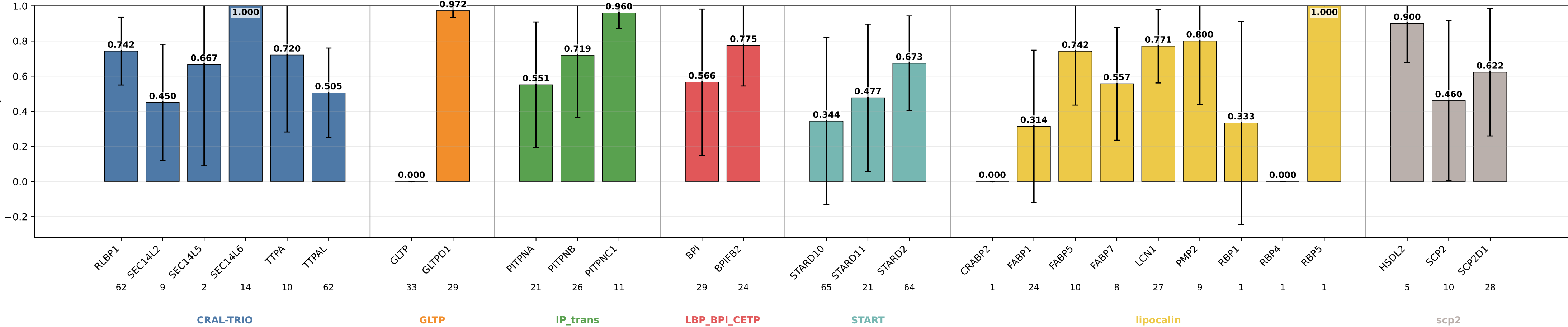
descriptors_head_family_neutral_lipprop_lambdasqrt sensitivity by subgroup descriptors_head_family_neutral_lipprop_lambdasqrt | class weights | lr=0.0001 | weight_decay=0.01 | final_m=4 | final_dropout=0.1 | hiddim=8 | heads=8 | batch=16 | ep=120 | seeds=0,1,2,3,4
