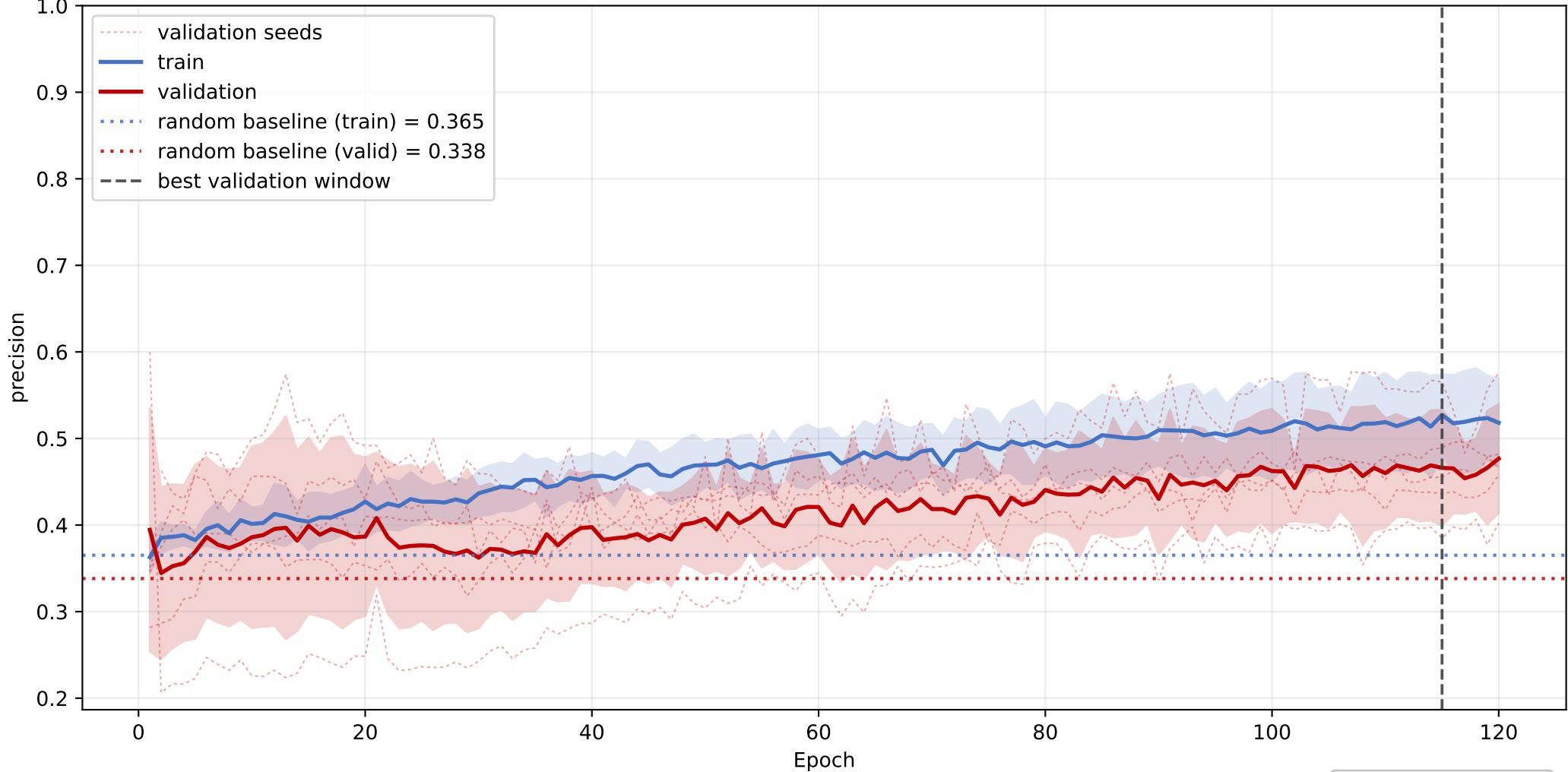
anionic: mean precision learning curve across seeds
