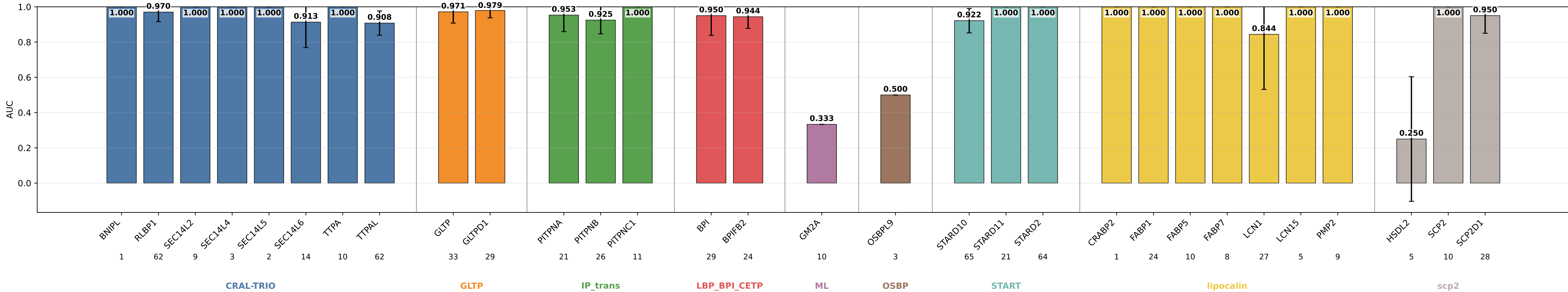
ge_s15_prothid32_hid64_noreg_forcedint AUC by subgroup ge_s15_prothid32_hid64_noreg_forcedint | class weights | lr=0.0001 | weight_decay=1e-05 | final_m=4 | final_dropout=0.0 | hiddim=64 | heads=8 | batch=16 | ep=120 | seeds=0,1,2,3,4
