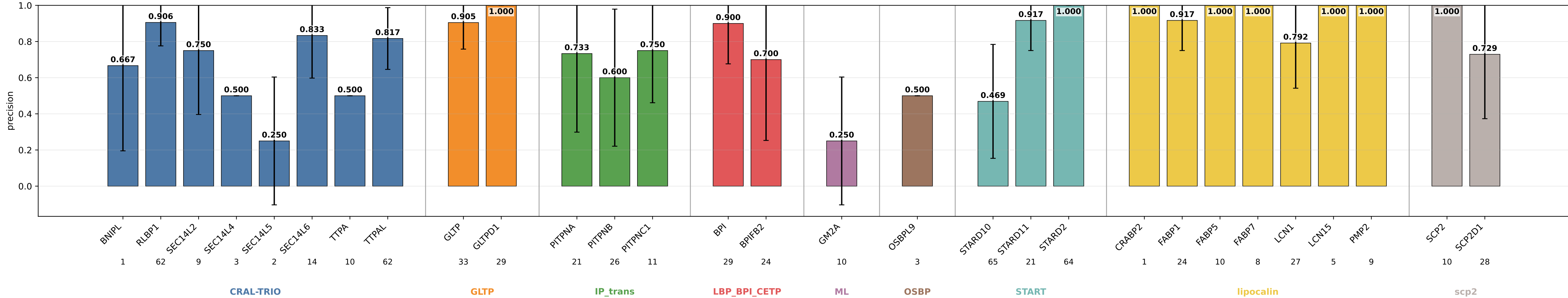
ge_s15_prothid32_hid64_noreg_nodebilin precision by subgroup ge_s15_prothid32_hid64_noreg_nodebilin | class weights | lr=0.0001 | weight_decay=1e-05 | final_m=4 | final_dropout=0.0 | hiddim=64 | heads=8 | batch=16 | ep=120 | seeds=0,1,2,3,4
