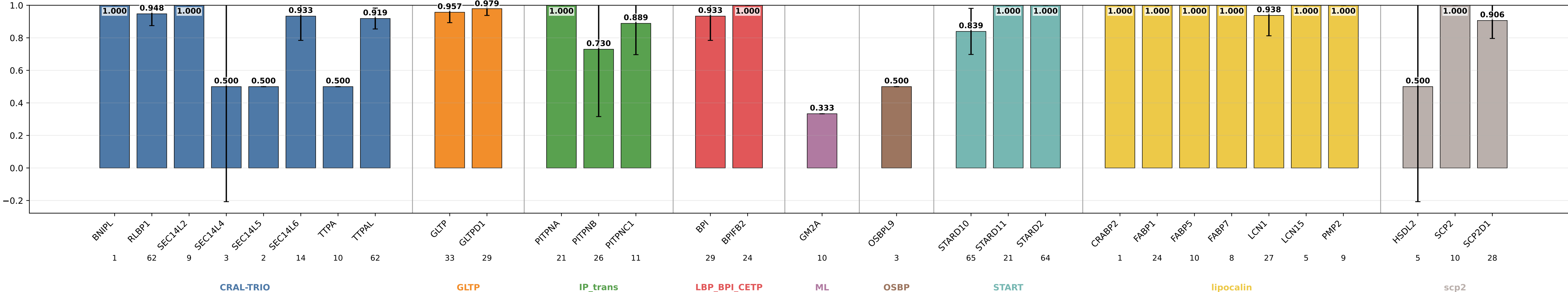
ge_s15_prothid32_hid64_noreg_nodebilinear AUC by subgroup ge_s15_prothid32_hid64_noreg_nodebilinear | class weights | lr=0.0001 | weight_decay=1e-05 | final_m=4 | final_dropout=0.0 | hiddim=64 | heads=8 | batch=16 | ep=120 | seeds=0,1,2,3,4
