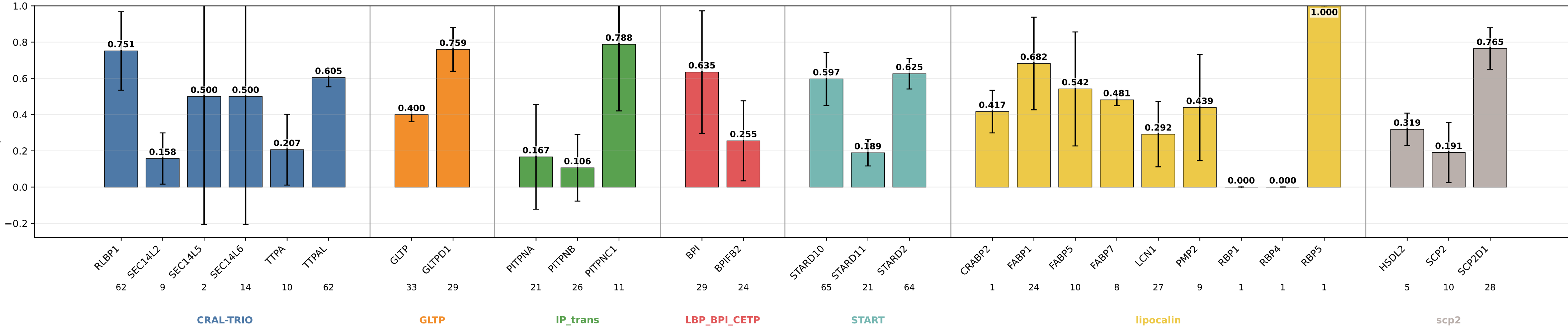
geometric_edge_mlp_protgeom8_lipid_class_targets precision by subgroup geometric_edge_mlp_protgeom8_lipid_class_targets | class weights | lr=0.0001 | weight_decay=0.01 | final_m=4 | final_dropout=0.1 | hiddim=8 | heads=8 | batch=16 | ep=120 | seeds=0,1,2
