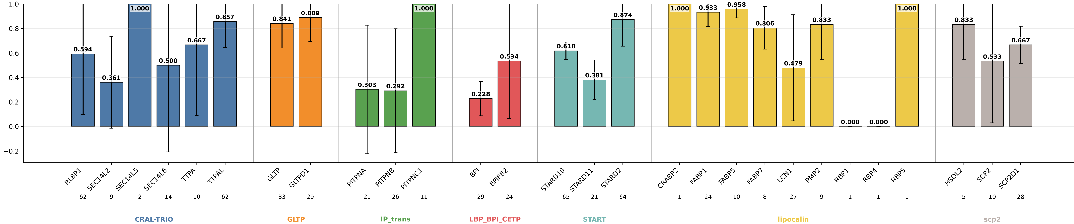
geometric_edge_mlp_protgeom8_lipid_class_targets sensitivity by subgroup geometric_edge_mlp_protgeom8_lipid_class_targets | class weights | lr=0.0001 | weight_decay=0.01 | final_m=4 | final_dropout=0.1 | hiddim=8 | heads=8 | batch=16 | ep=120 | seeds=0,1,2
