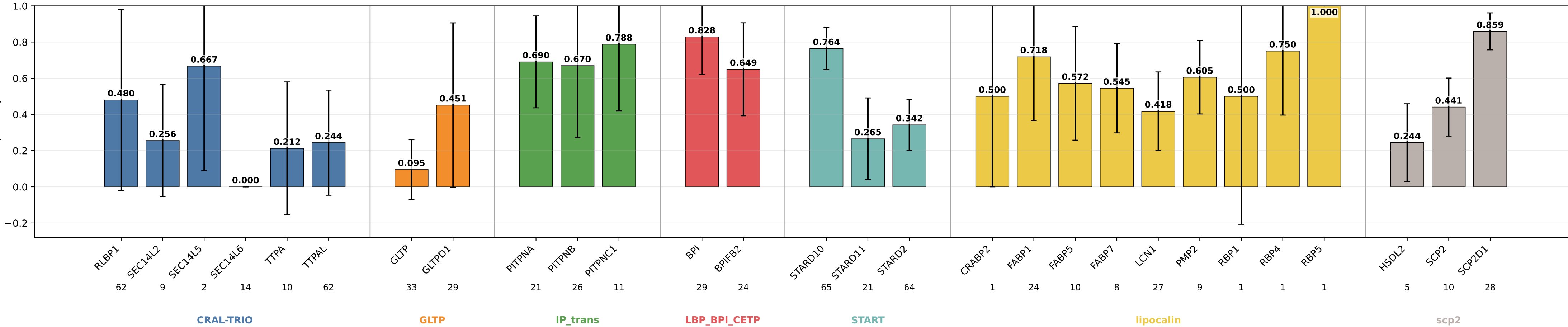
geometric_edge_mlp_protgeom8_lipid_class_targets specificity by subgroup geometric_edge_mlp_protgeom8_lipid_class_targets | class weights | lr=0.0001 | weight_decay=0.01 | final_m=4 | final_dropout=0.1 | hiddim=8 | heads=8 | batch=16 | ep=120 | seeds=0,1,2
