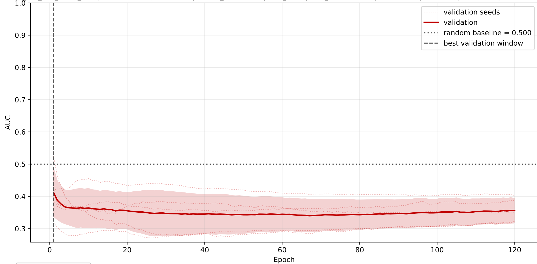
PC: mean AUC learning curve across seeds
