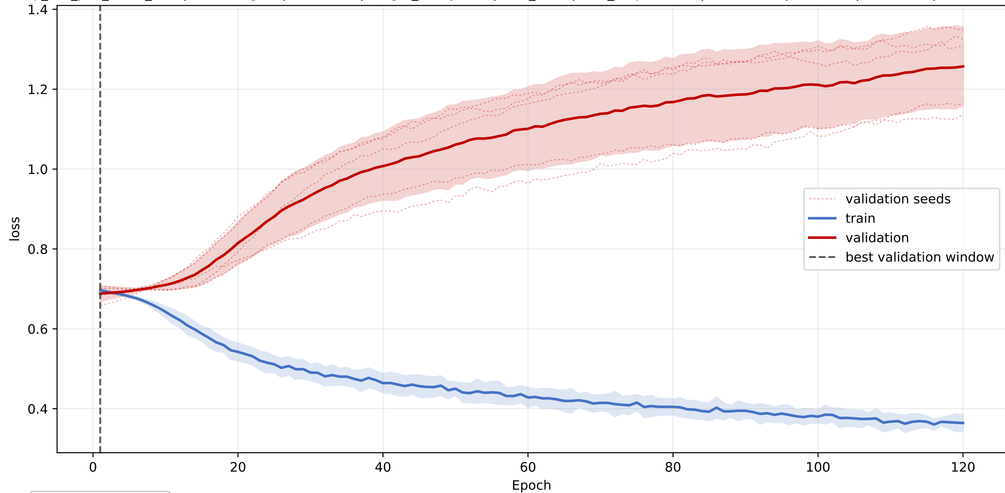
PC: mean loss learning curve across seeds
