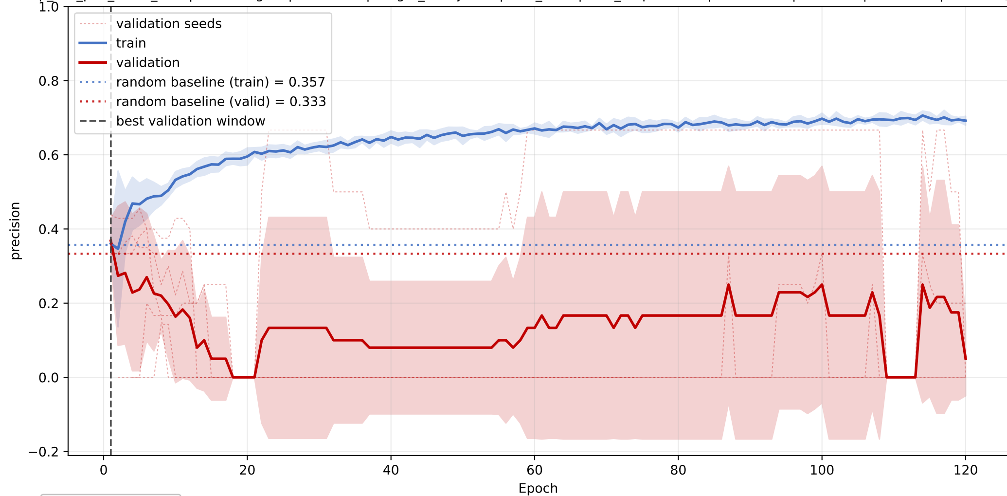
PI: mean precision learning curve across seeds
