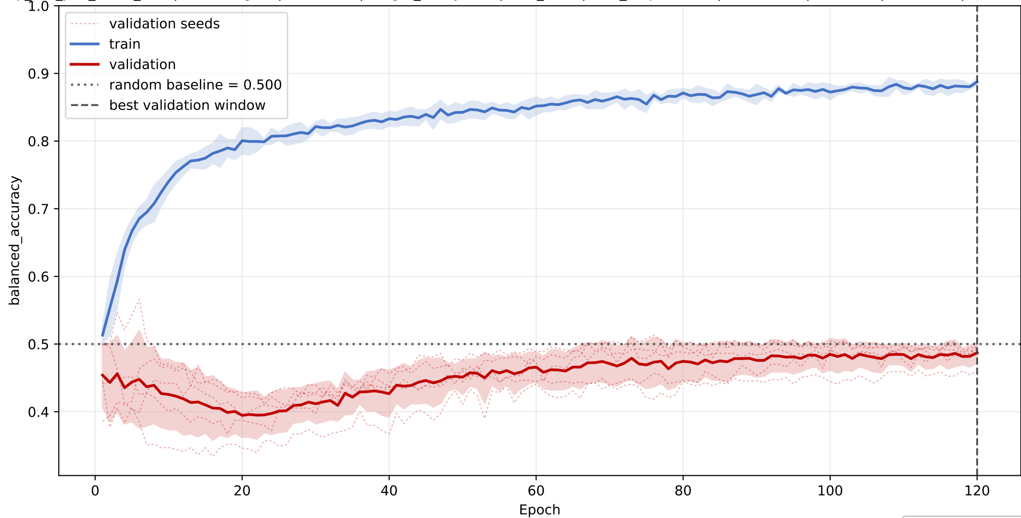
PC: mean balanced_accuracy learning curve across seeds
