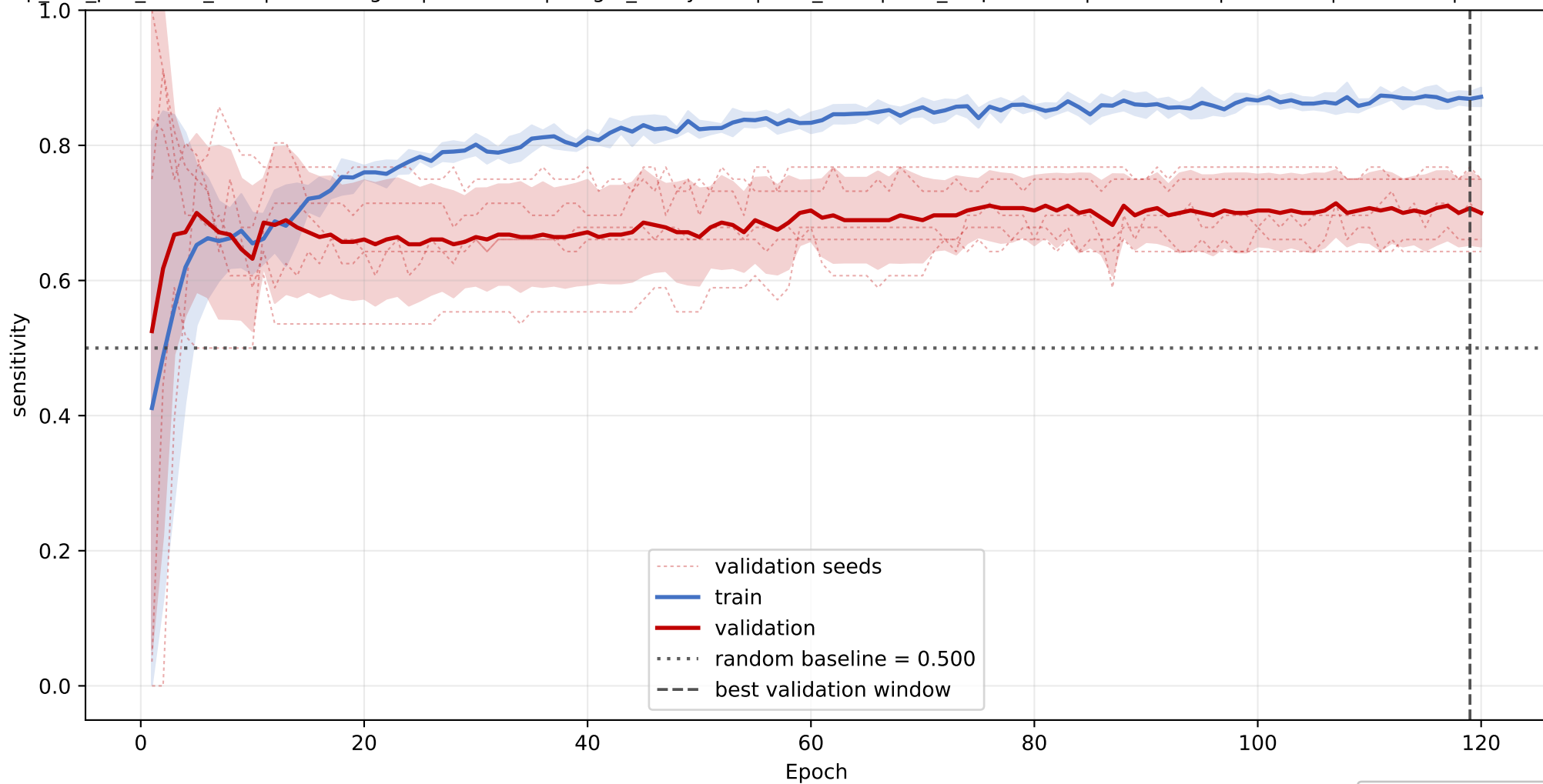
PG: mean sensitivity learning curve across seeds
