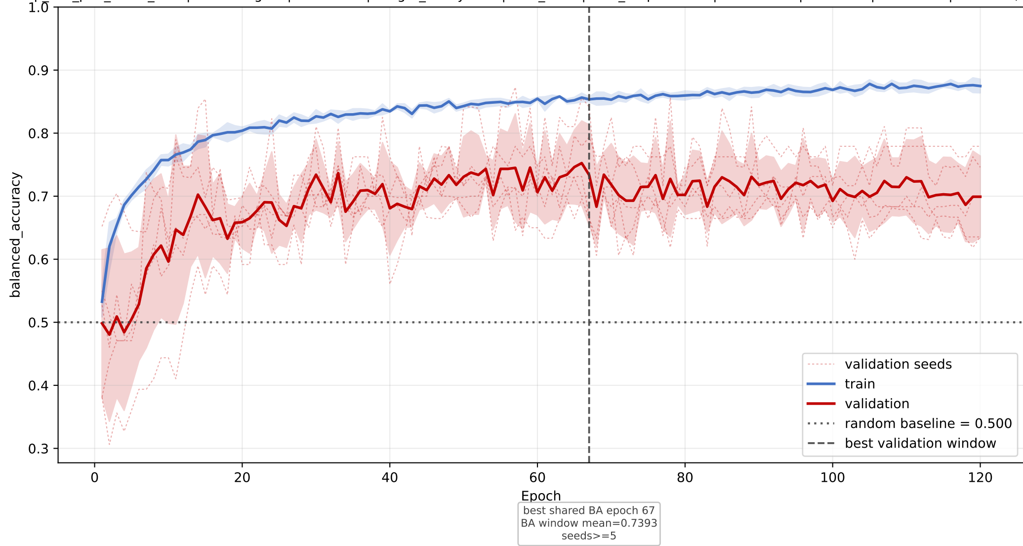
LPC+LPE+LPG: mean balanced_accuracy learning curve across seeds
