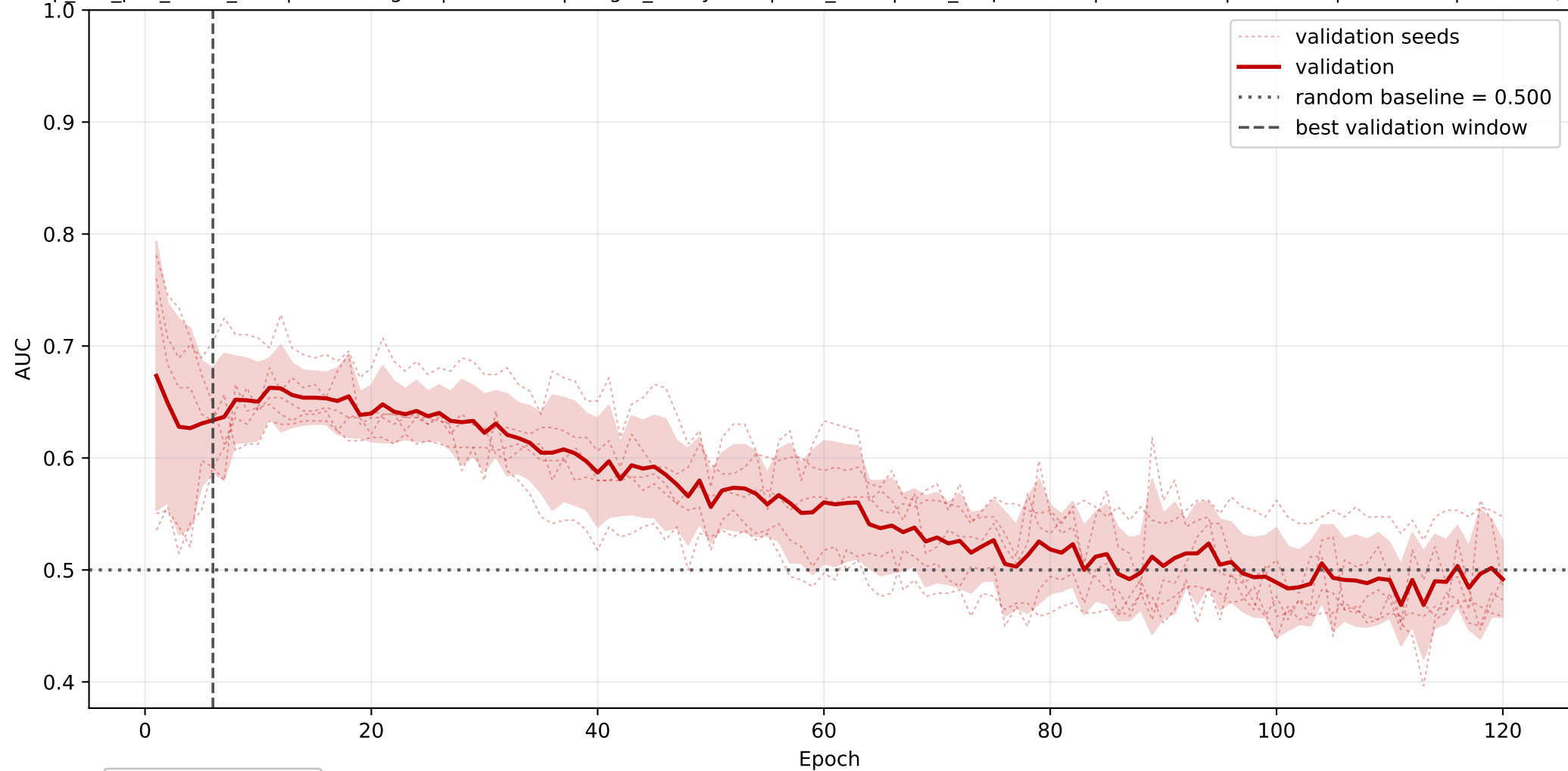
PA: mean AUC learning curve across seeds
