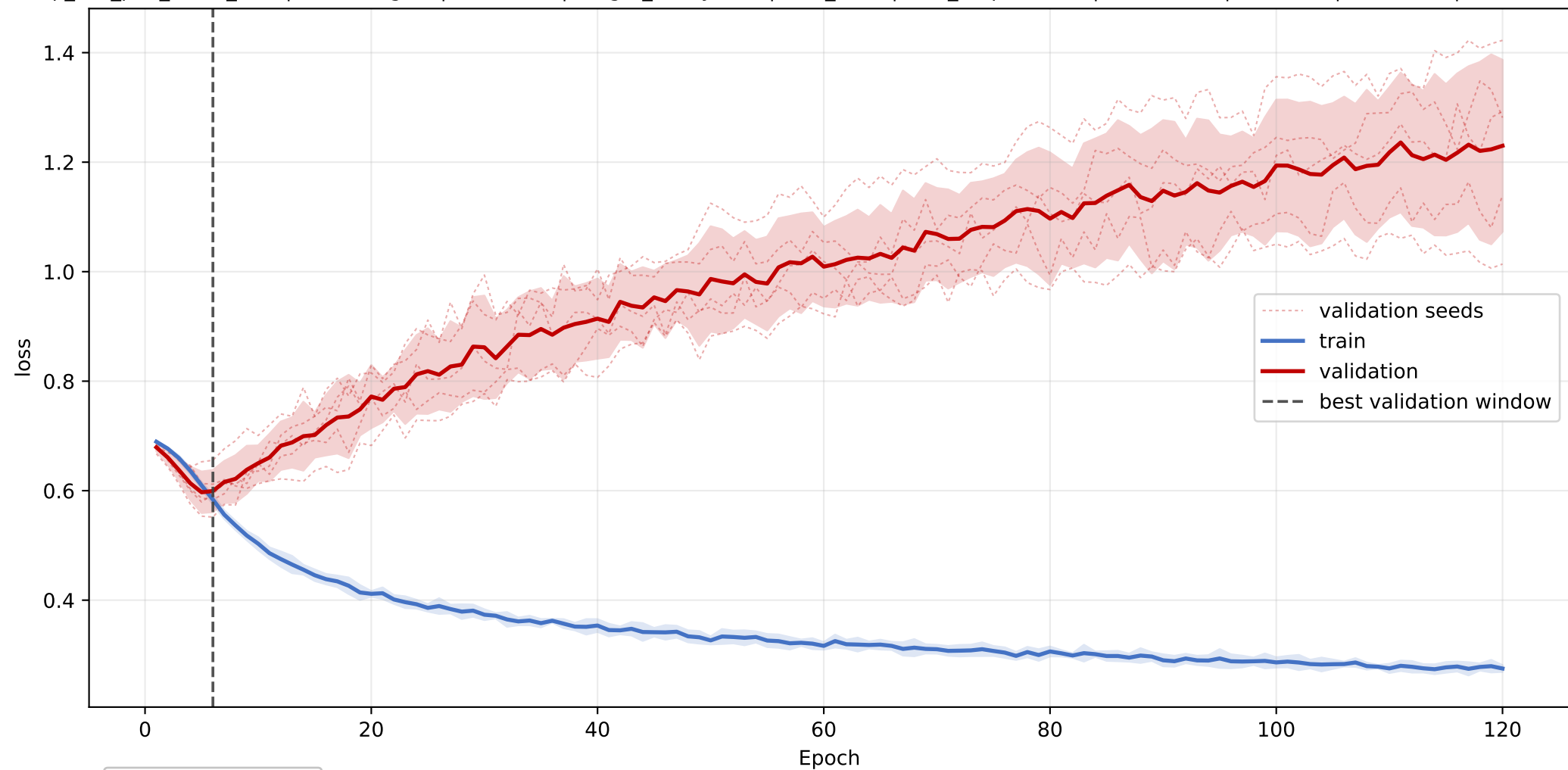
PA: mean loss learning curve across seeds
