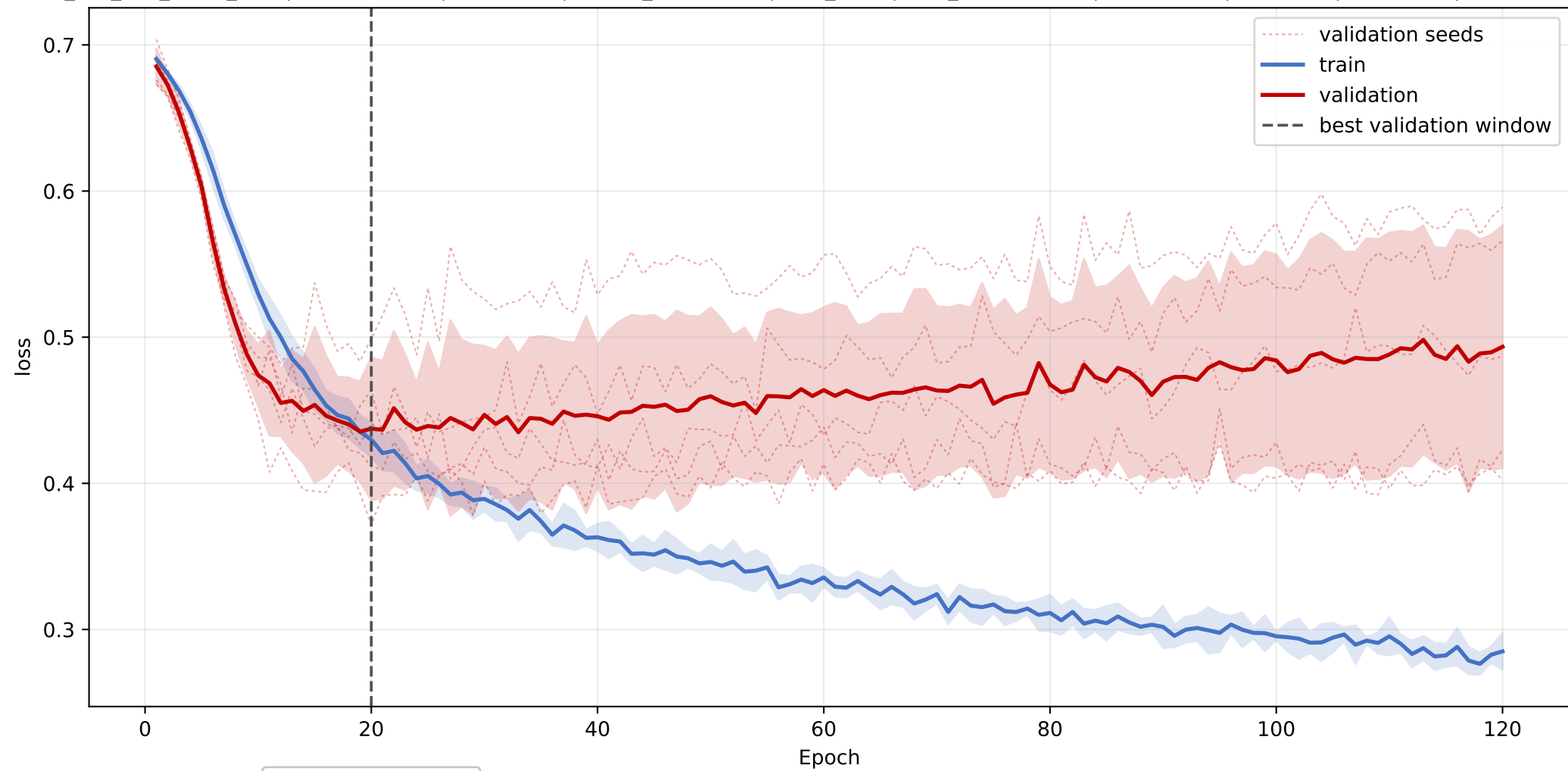
PE: mean loss learning curve across seeds
