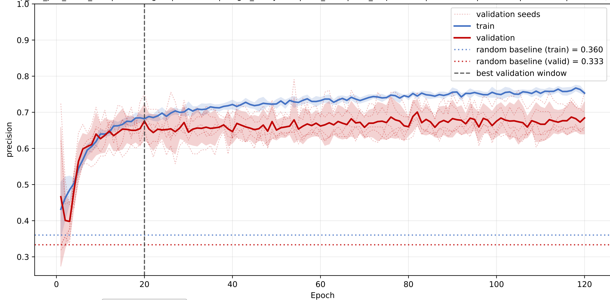
PE: mean precision learning curve across seeds
