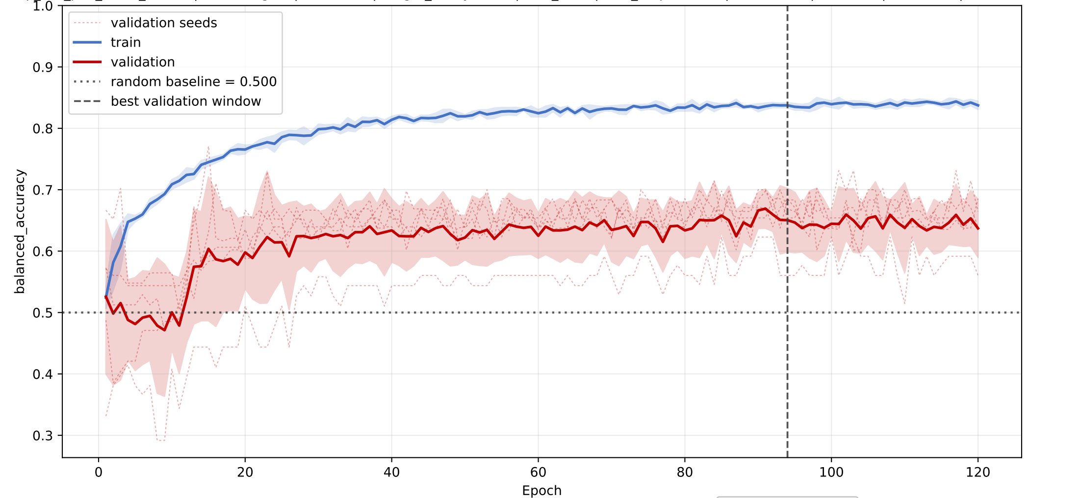
LPC+LPE+LPG: mean balanced_accuracy learning curve across seeds
